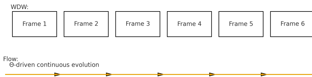
Figure A1. Discrete frames versus \Theta -driven continuity. WDW captures static frames; the time field provides the physical medium for motion between them.
