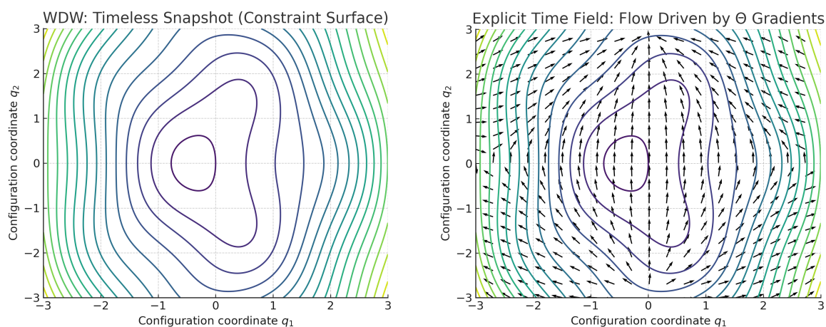
(a) Wheeler–DeWitt: timeless snapshot. The Hamiltonian acts as a constraint; no generator of motion.
