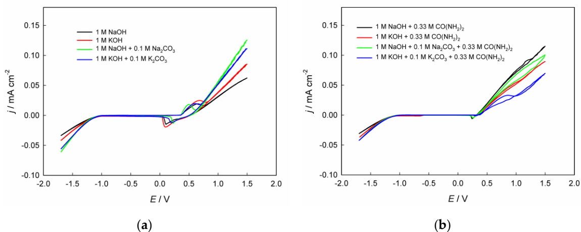
Figure 2. CVAs recorded in solutions of different compositions: (a) without added urea; (b) with urea added to the solution.
