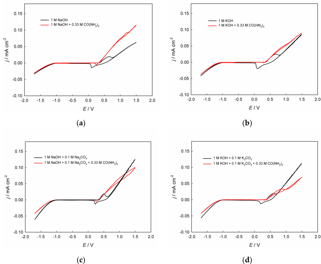
Figure 1. CVAs recorded in solutions of different compositions (as indicated in the figure).
