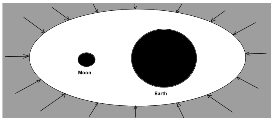
Figure 1. Gravitational force is pushing force of dark energy.
