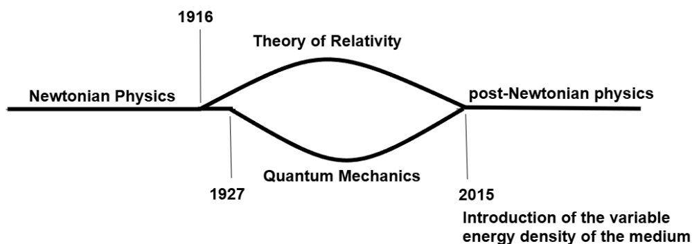
Figure 11. Development of physics in last 100 years.
