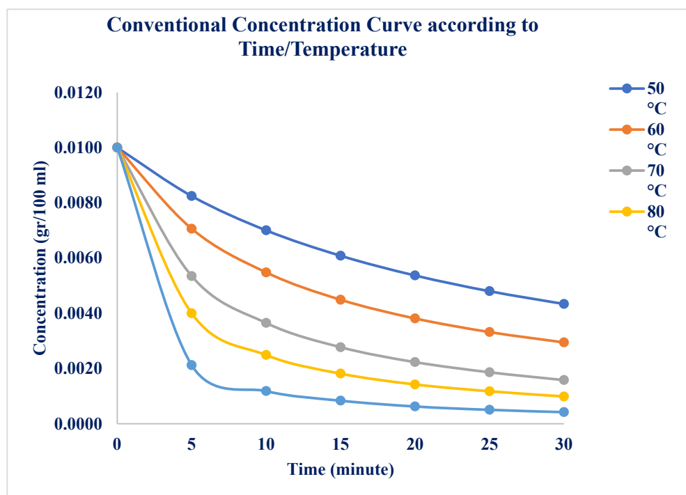
Figure 4. Effect of Time and Temperature on Dye Concentration (Conventional Heating).
