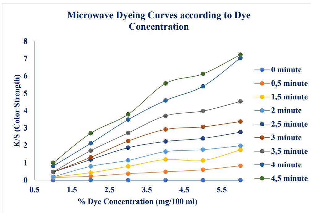
Figure 10. Effect of Dye Concentration at Different Reaction Times (Microwave Heating).
