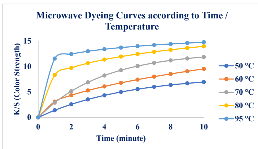
Figure 8. Effect of Time and Temperature on Color Strength (Microwave Heating).
