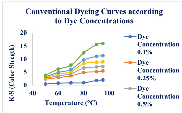
Figure 6. Effect of Temperature at Different Concentrations (Conventional Heating).
