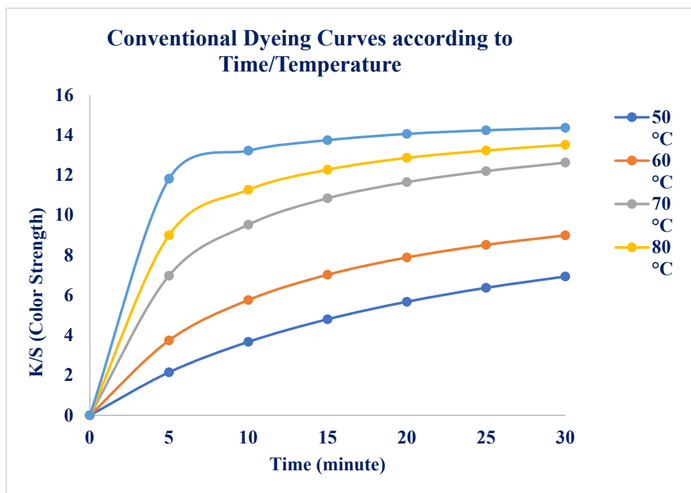
Figure 3. Effect of Time and Temperature on Color Strength (Conventional Heating).
