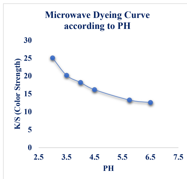
Figure 7. Effect of PH (Microwave Heating).
