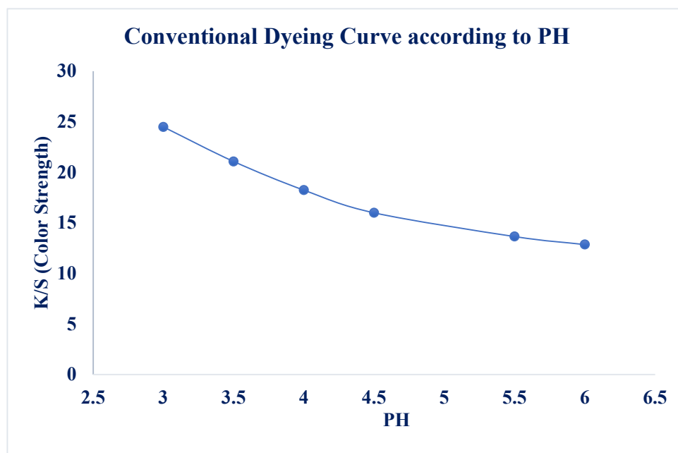
Figure 2. Effect of PH (Conventional Heating).
