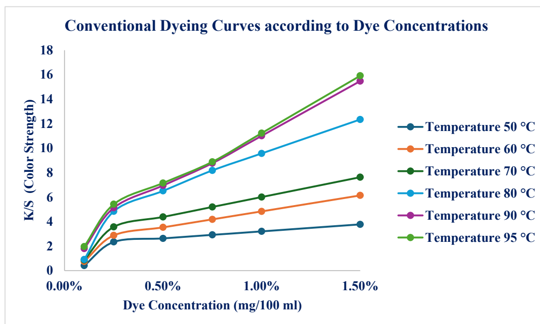
Figure 5. Effect of Dye Concentration at Different Temperature (Conventional Heating).
