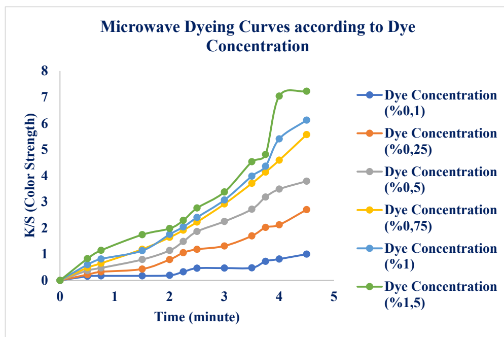
Figure 11. Effect of Reaction Time at Different Concentrations (Microwave Heating).
