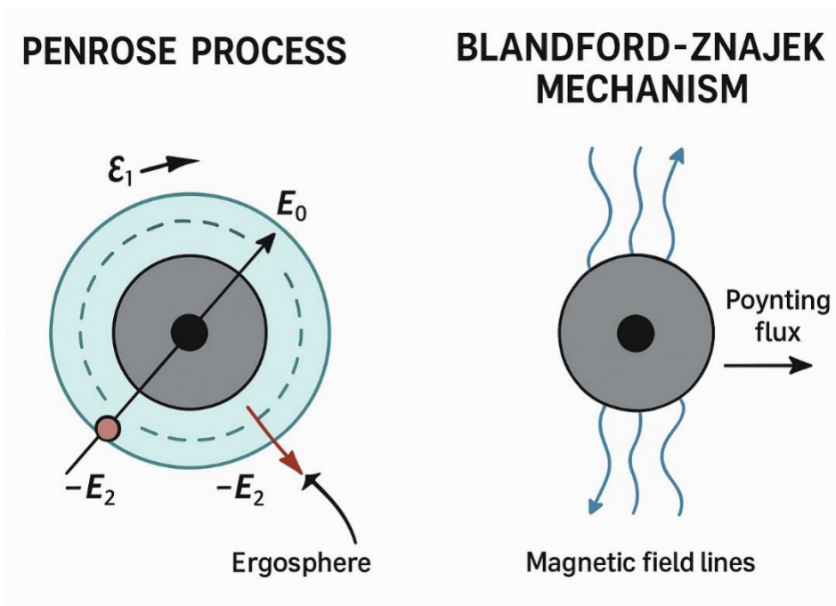
Figure 1. Penrose Process vs. Blandford-Znajek Mechanism
