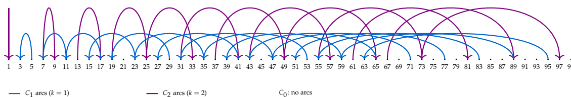
Figure A1. Reverse Collatz Coverage with Minimal Lifts ( k = 1, 2 )
