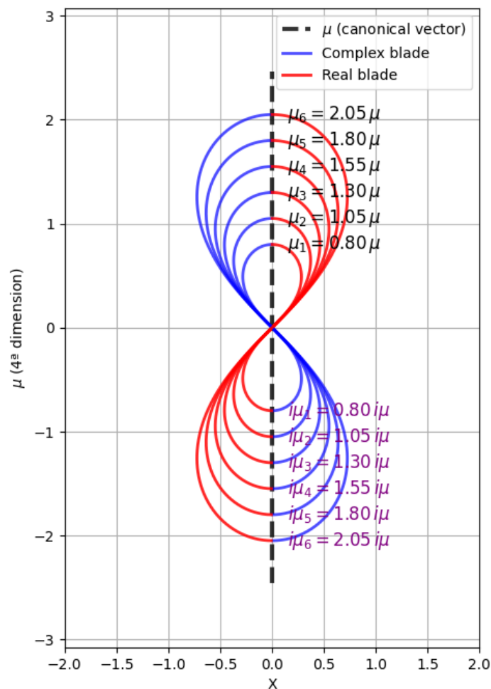
Figure 1. Geometric representation of Alpha group space in \mathbb{R}^4 (Poincaré cut), illustrating a topological structure exhibiting anisotropy.
