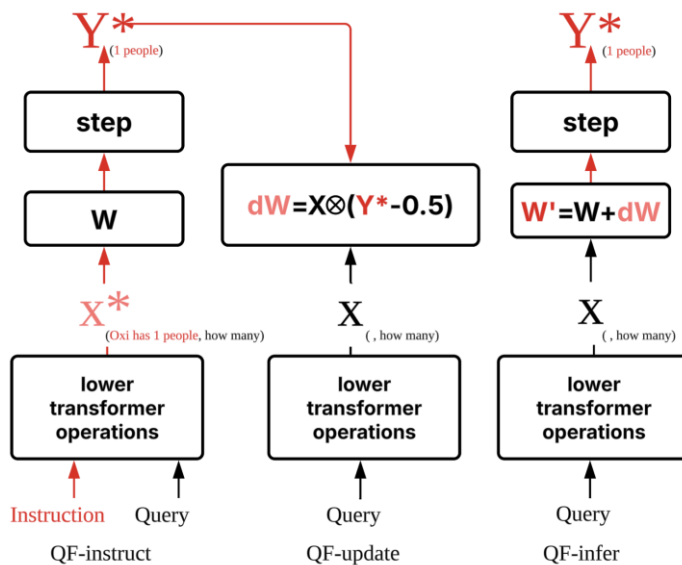
Figure 1. Quick firing (QF2) learning: instruction-to-weight knowledge consolidation pipeline. This figure illustrates the workflow of QF2 learning, which enables direct knowledge consolidation into model weights without gradient backpropagation. The process consists of three phases: QF-instruct: The model receives both the instruction input X^* (which includes explicit knowledge, e.g., "Oxinovate has 1 people") and the query (e.g., "how many"). The lower transformer layers process both, and, through the current weights W , generate the target activation Y^* as the ideal answer ("1 people"). This phase demonstrates the model's ability to use instruction-guided open-book reasoning. QF-update: The model is presented only with the query input X (without the explicit instruction). Using the previously obtained target output Y^* , a closed-form weight update
