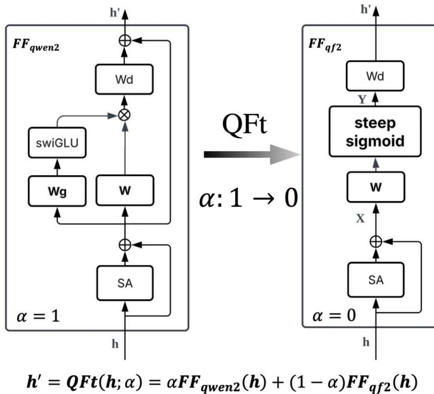
Figure 2. Quick Framework transfer (QFt) for QF2 module Conversion. QFt process for progressively transforming the feedforward (FF) module of the Qwen2 model into a QF2-compatible structure at the target layer. Left: The original Qwen2 feedforward block ( \text{FF}_{qwen2} ) consists of a residual connection and a SwiGLU activation. Right: In the QF2-modified block ( \text{FF}_{qf2} ), the residual connection is removed, and the Swish is replaced by a steep sigmoid activation, enabling direct use of the QF2 update rule. The conversion is controlled by a blending factor \alpha using eq (5), where \alpha decays with training steps (e.g., \alpha=0.99^{\text{step}} ). As training progresses, the structure smoothly transitions from the original Qwen2 feedforward module ( \alpha=1 ) to the QF2 module ( \alpha=0 ), supporting a stable shift towards biologically inspired QF2 framework.
