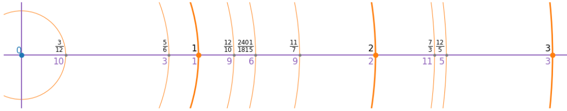
Figure 3. Few examples of rational numbers q \in \mathbb{Q}_{13} in a finite framed field \mathbb{Z}_{13}(0, 1) . Note the pseudo-rational numbers 6/5 , 12/10 as well as 11/7 that all represent the exact same element 9 \in \mathbb{Z}_{13}(0, 1) .
