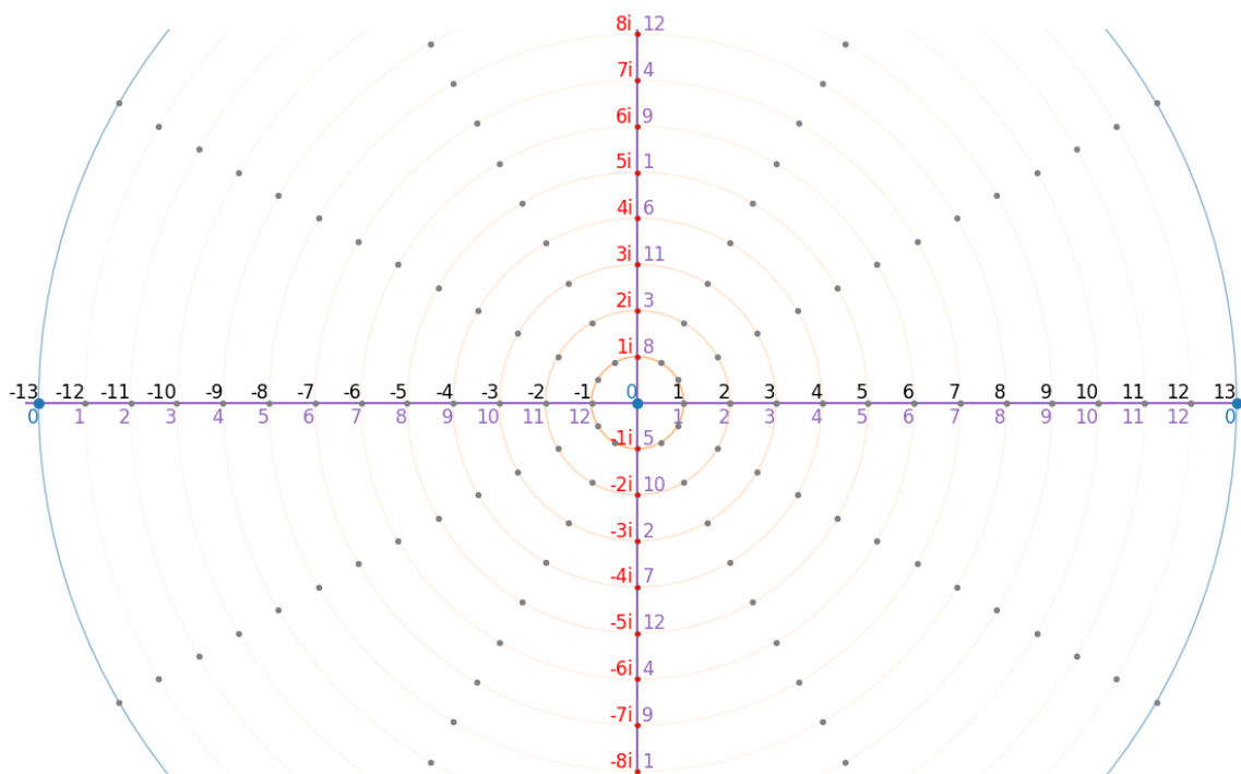
Figure 5. Pseudo-complex numbers plane \mathbb{C}_p in a finite framed field \mathbb{Z}_{13}(0,1) . Horizontal axis represents the pseudo-reals \mathbb{R}_p on the prime meridian and the vertical axis represents the imaginary numbers c = z \cdot i indicated by their respective red labels. The corresponding elements k(c) are depicted in purple. The blue line indicates the periodicity of the finite field.
