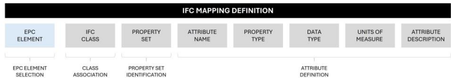
Figure 4. IFC Mapping structure.
