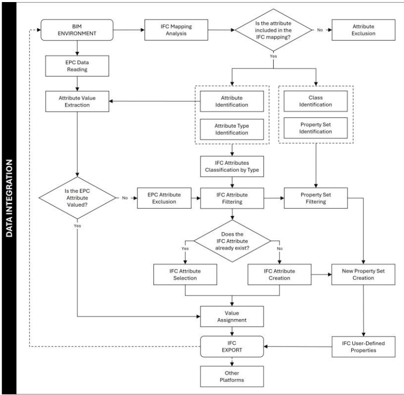
Figure 6. Workflow for the data integration.
