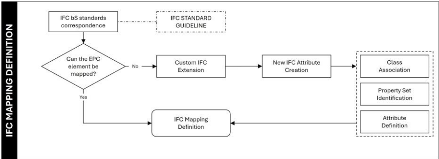
Figure 5. Workflow for the IFC Mapping definition.
