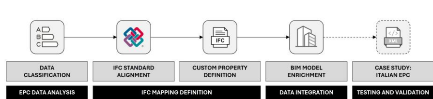
Figure 2. Methodology schema.
