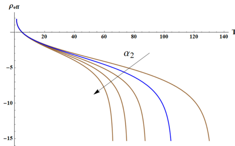
Figure 8. Here are curves \rho_{eff}(T; \alpha_2 \in \{0.04, 0.05 \text{ (Blue)}, 0.06, 0.07, 0.08\}, \omega = 2.3) . The asymptotic behavior corresponds to T = \frac{\omega^2}{\alpha_2} . Black arrow depicts the increase in \alpha_2 .
