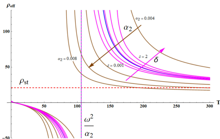
Figure 5. The plots demonstrate change in the resonance curves when parameters \alpha_2 and \delta are varied.
