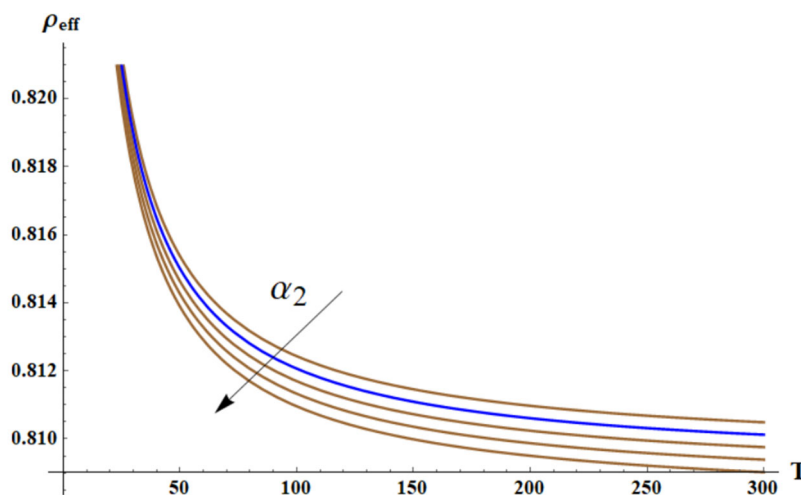
Figure 7. Curves \rho_{eff}(T; \alpha_2 \in \{0.04, 0.05 \text{ (Blue curve)}, 0.06, 0.07, 0.08\}, \omega = 2.3) are depicted. Black arrow depicts the increase in \alpha_2 . \lim_{T \rightarrow \infty} (\rho_{eff}(T, \omega)) = 1 + \frac{1}{\alpha_2 - \omega^2} .
