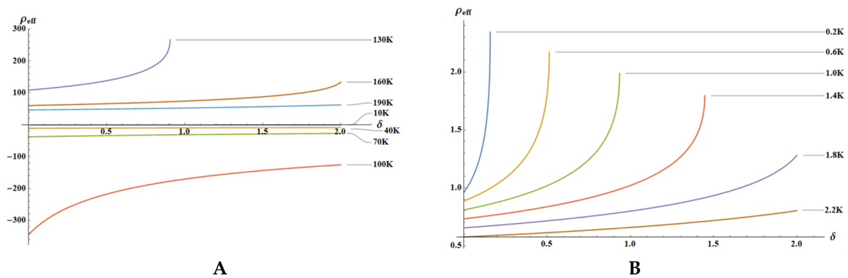
Figure 6. A. The dependence \rho_{eff}(\delta) is depicted for various temperatures T . curves \rho_{eff}(\delta; \omega = 2.3, \alpha_2 = 0.05, T \in [0.2, 190]) are depicted. B. As \delta and T tend to zero \rho_{eff} (for the dimensionless parameters) tends to 1, as it is expected from Eq. 15.
