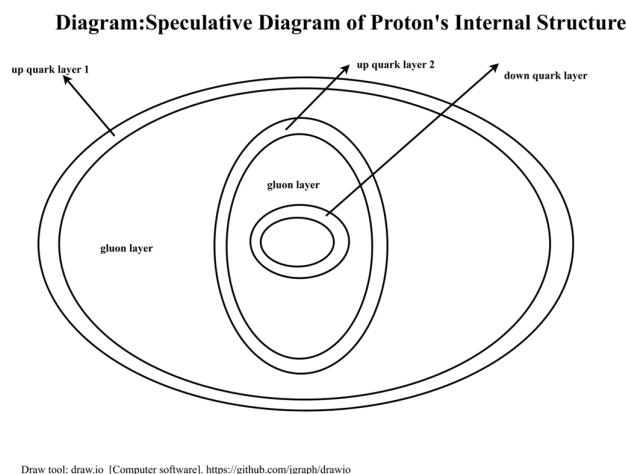
Figure A1. Speculative Diagram of Proton's Internal Structure with Quarks and Gluons. Online Draw tool [25].
