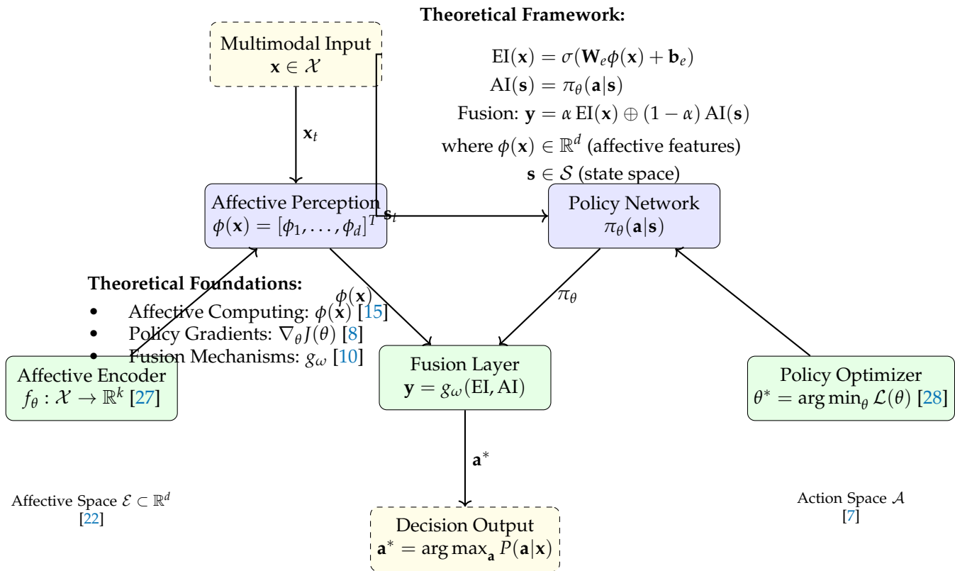
Figure 3. Formal architecture for EI-AI integration showing: (1) Affective perception pipeline, (2) Cognitive reasoning pathway, and (3) Hybrid fusion mechanism. The mathematical framework combines deep learning ( f_\theta ) with reinforcement learning ( \pi_\theta ) through differentiable fusion g_\omega .
