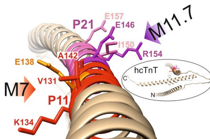
Figure 7. Ribbon cartoon of the hcTnT backbone structure model. The alpha helix which contains the M7 (red) and the M11.7 (pink) epitopes is shown. Selected amino acid residues are shown (stick models) and labeled (single letter code). Amino acid residues E138 (orange), E146 (purple) and R154 (purple) are required for antibody binding. The orientations of antibody docking are indicated with red (M7) and purple (M11.7) arrows. A ribbon structure model of full-length hcTnT (Uniprot accession no.: P45379) is shown as insert (circled). N- and C-termini are labeled.
