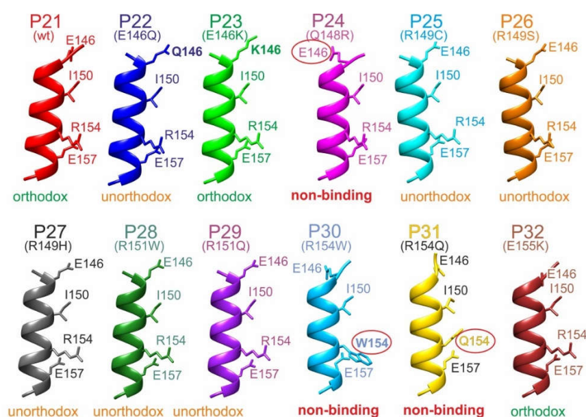
Figure 6. Ribbon cartoons of M11.7 epitope peptide backbone structure models. Alpha helices of P21 to P32 are shown from side. Selected amino acid residues are shown (stick models) and labeled (single letter code). Wild type (wt) and amino acid exchanges (point mutations) are indicated in parentheses. Amino acid numbering as in the full-length hcTnT protein. Binding modes with the M11.7 antibody are given at the bottom. Amino acid residues which prevent binding are circled. The “E-I-R-E” binding motif amino acid residues are shown.
