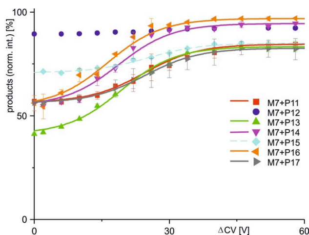
Figure 3. Courses of normalized product ion intensities of M7 antibody - epitope peptide complexes as functions of collision cell voltage differences ( \Delta CV ). The immune complex dissociations with peptides P11 (red square), P12 (violet dot), P13 (green triangle), P14 (violet triangle), P15 (light blue diamond), P16 (orange triangle), and P17 (grey triangle) are shown. Each data point is the mean of two independent measurements (see Tables S3). Vertical bars indicate standard deviations. The sigmoidal shaped curves were fitted using a Boltzmann function. Solid lines indicate orthodox binding. Dotted lines indicate unorthodox binding. Curve parameters are given in Table 2.
