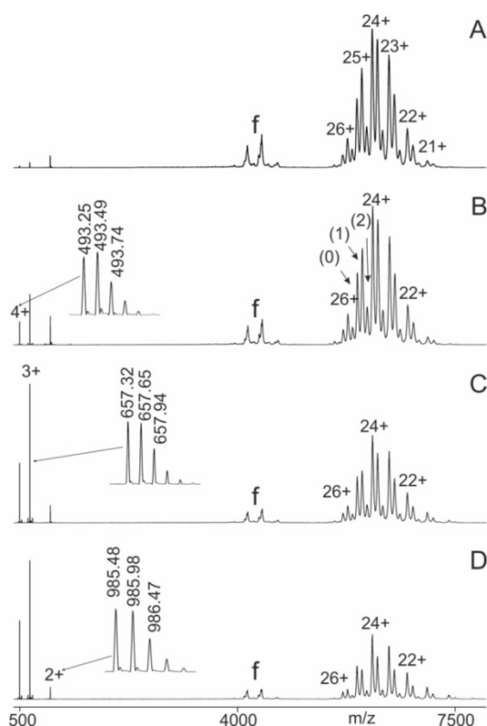
Figure 2. Nano-ESI mass spectra of peptide 21 (AEQQRIRNEREKERQ) – M11.7 antibody mixtures with increasing collision cell voltage differences ( \Delta CV ). A: 2 V, B: 14 V, C: 30 V, D: 52 V. Charge states are given for the ion signals (right ion series) of the antibody (0) and the immune complexes (antibody plus one peptide (1)
