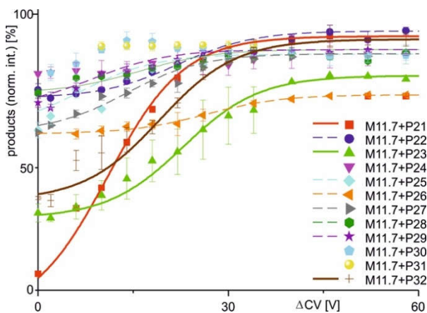
Figure 4. Courses of normalized product ion intensities of M11.7 antibody - epitope peptide complexes as functions of collision cell voltage differences ( \Delta CV ). The immune complex dissociations with peptides P21 (red square), P22 (violet dot), P23 (green triangle), P24 (violet triangle), P25 (light blue diamond), P26 (orange triangle), P27 (grey triangle), P28 (green hexagon), P29 (purple star), P30 (cyan pentagon), P31 (yellow dot), and P32 (brown cross) are shown. Each data point is the mean of two independent measurements (see Table S4). Vertical bars indicate standard deviations. The sigmoidal shaped curves were fitted using a Boltzmann function. Solid lines indicate orthodox binding. Dotted lines indicate unorthodox binding. Curve parameters are given in Table 2.
