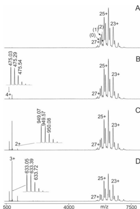
Figure 1. Nano-ESI mass spectra of peptide 11 (LVSLKDRIERRRAER) – M7 antibody mixtures with increasing collision cell voltage differences ( \Delta CV ). A: 2 V, B: 14 V, C: 30 V, D: 52 V. Charge states are given for the ion signals (right ion series) of the antibody (0) and the immune complexes (antibody plus one peptide (1) and antibody plus two peptides (2)). Charge states for peptide ion signals are given on the left. The insets in B, C, and D show zoom views of the isotopically resolved peptide ion signals and their m/z values. The quadrupole was set to block transmission of ions < m/z 3850. Molar ratio of peptide to antibody was 2.1 : 1. Solvent: 200 mM ammonium acetate, pH 6.7.
