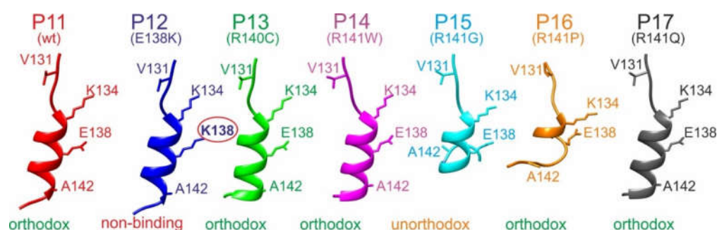
Figure 5. Ribbon cartoons of M7 epitope peptide backbone structure models. Alpha helices of P11 to P17 are shown from side. Selected amino acid residues are shown (stick model) and labeled (single letter code). Wild type (wt) and amino acid exchanges (point mutations) are indicated in parentheses. Amino acid numbering as in the full-length hcTnT protein. Binding modes with the M7 antibody are given at the bottom. Amino acid residues which prevent binding are circled. The “V-K-E-A” binding motif amino acid residues are shown.
