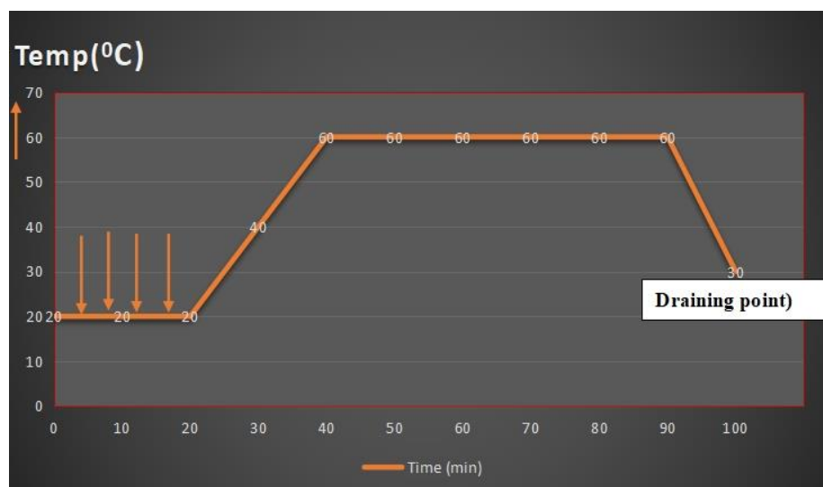
Figure 2. Temperature VS Time Graph of Dyeing process.
