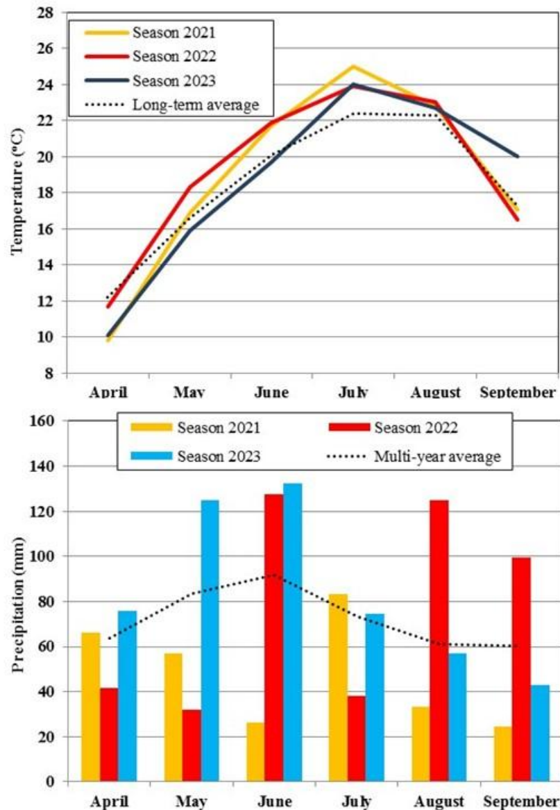
Figure 1. Monthly averages of air temperatures and precipitation during the three investigated seasons (2021–2023) and long-term average (1990–2019) (dotted line); data were obtained from the meteorological station in Kraljevo, about 2 km from the experimental field. .
