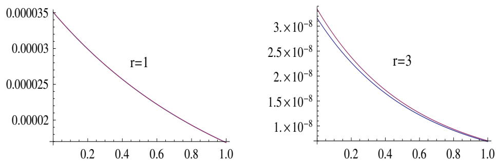
Figure 4. The graphs of the functions x \mapsto D_{r,5}(x, 4, \pi) \mp \tilde{\delta}_5(x, 4) \approx \delta_r(x, 4, \pi) .
