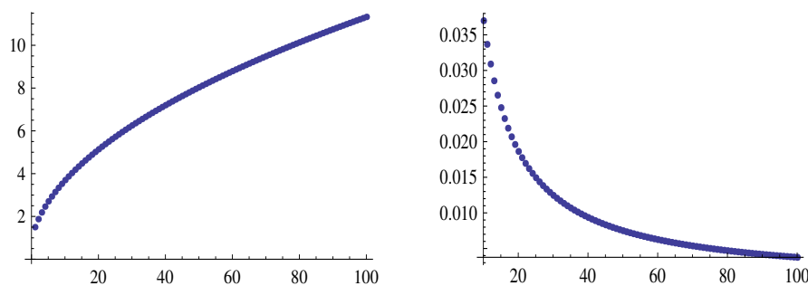
Figure 7. The graphs of the sequences \left| \left(-\frac{3}{2}\right)_n \right| and \frac{\left| \left(-\frac{3}{2}\right)_n - b_1(n) \right|}{|b_1(n)|} , left and right respectively.
