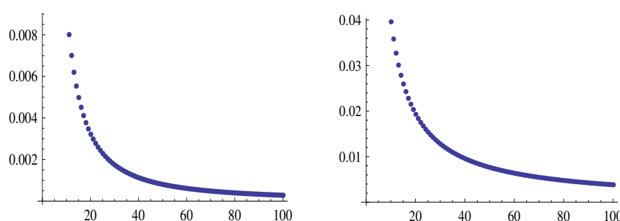
Figure 9. The graphs of the sequences \left|\binom{\frac{1}{2}}{n}\right| and \left|\binom{\frac{1}{2}}{n} - b_3(n)\right|/|b_3(n)| , left and right respectively.
