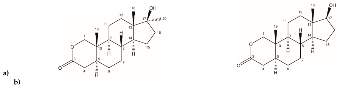
Figure 1. Structure of 2-oxa steroids. (a) 17 \beta -hydroxy-17 \alpha -methyl-2-oxa-5 \alpha -androstan-3-one – Oxandrolone ( 1 ); (b) 17 \beta -hydroxy-2-oxa-5 \alpha -androstan-3-one ( 6 ).
