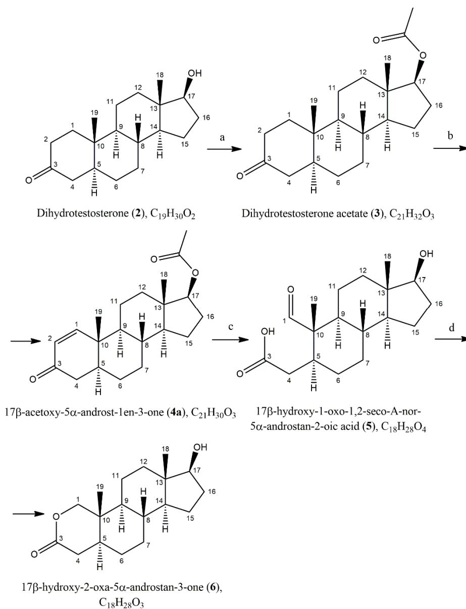
Scheme 2. Synthesis of 17β-hydroxy-2-oxa-5α-androstan-3-one ( 6 ). Reaction conditions: a) Ac 2 O, pyridine, 24h; b) DDQ, dioxane; c) KMnO 4 /NaIO 4 , Na 2 CO 3 , i-PrOH/H 2 O; d) NaBH 4 , NaOH, H 2 O.
