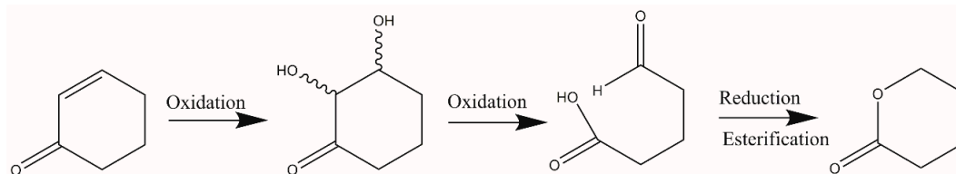
Scheme 1. General procedure for the synthesis of lactones from the corresponding \alpha,\beta -unsaturated ketone.
