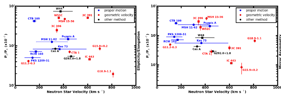
Figure 4. Quadrupole (left) and octupole (right) power ratios are plotted against NS velocities for a sample of SNRs [75]. Blue points indicate velocities obtained through proper motion measurements, while red points show velocities determined by the geometric method.
