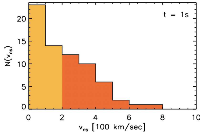
Figure 3. The histograms display the velocity distribution of NSs for the 70 models detailed in Tables A.1–A.5 of [74]. The solid black line represents the velocity distribution at t = 1 s. The darker shaded region indicates the subset of models where NSs attain velocities exceeding 200 km/s within one second of the core bounce.
