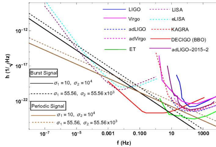
Figure 2. The variation of GW intensity with radiation frequency is presented, illustrating a pulsar kick driven by asymmetric neutrino emission induced by ultralight DM [58]. Sensitivity curves of GW detectors are included for reference.
