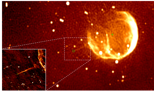
Figure 1. The pulsar kick of radio pulsar PSR J0002+6216 is indicated by a tail-like structure relative to the surrounding nebula [32]. This structure was captured in images from the Very Large Array (VLA), with timing analysis conducted by Fermi.
