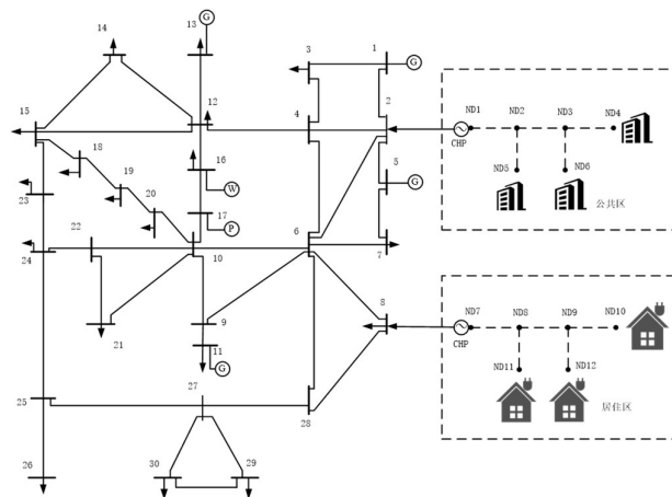
Figure 3. System Structure Diagram.
