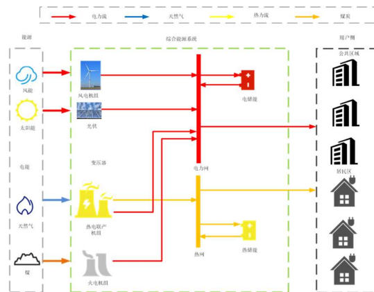
Figure 1. An integrated electric heating energy system model considering the difference of multi-district heating.
