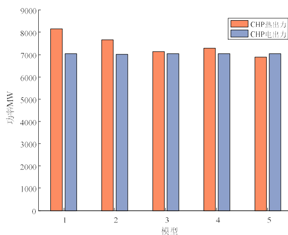
Figure 5. Electric and Thermal Output of Five Model CHP Units.
