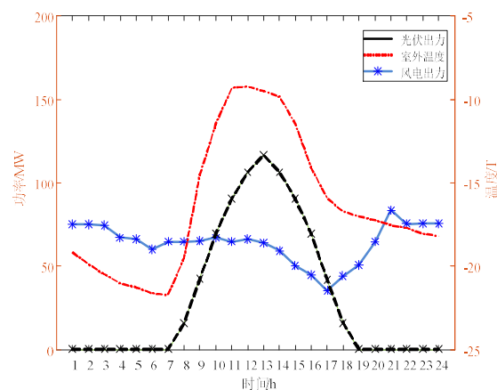
Figure 4. Curve of Wind and Solar Output and Outdoor Temperature.
