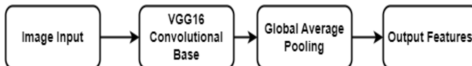
Figure 6. Architecture of the NFE Model.
