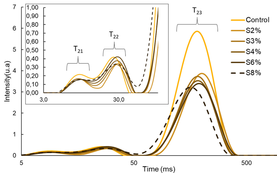
Figure 2. Distributions of the relaxation time after inverse Laplace transform analysis of LF-NMR spectra of the cellulose-based gels formulated with 0, 2, 3, 4, 6 and 8 % CRF.
