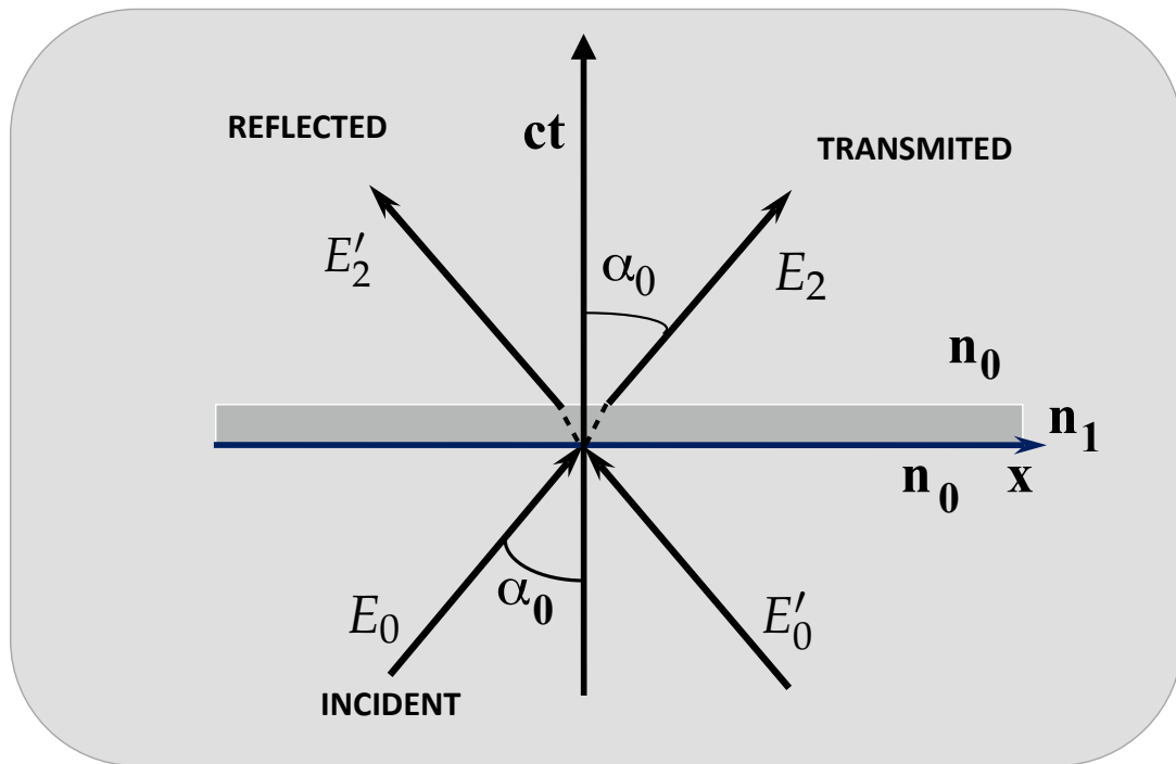
Figure 3. Temporal beam-splitter, made of two successive time-refraction events: First, at t = 0 the refractive index suddenly changes, from n_0 to n_1 , and then at t = \tau > 0 , the refractive index returns to its initial value n_0 . Incident, reflected and transmitted rays across the temporal slab of duration \tau are represented.
