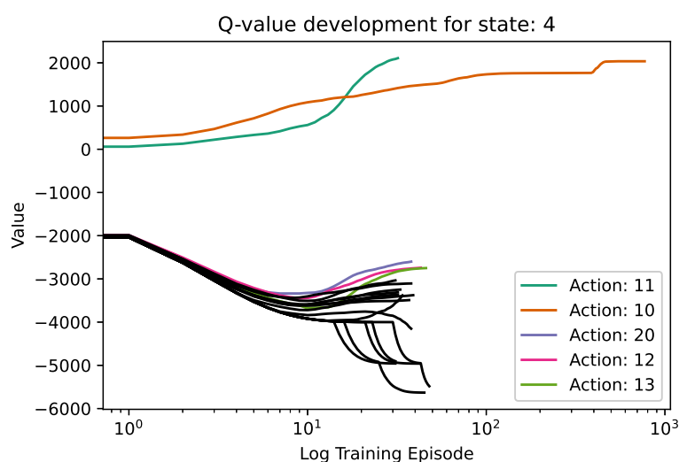
Figure 5. Non-chronological Q-value development during the training process for all potential actions in State 4
