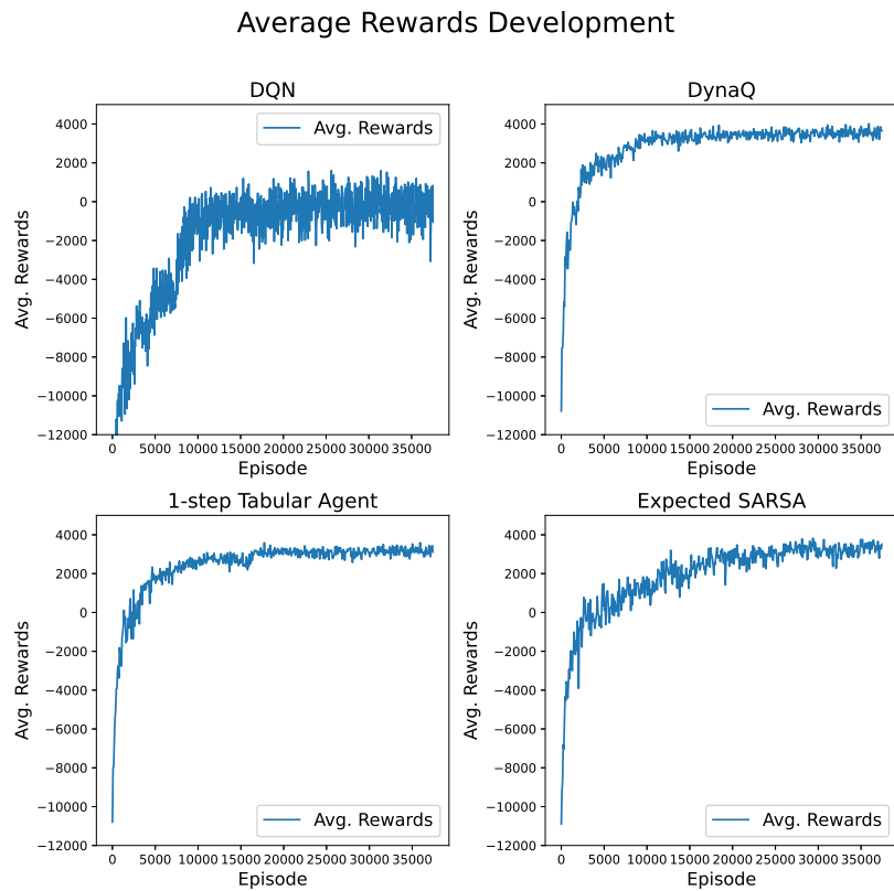
Figure 4. Comparison of average rewards development during training on non-random rewards for DQN and tabular agents
