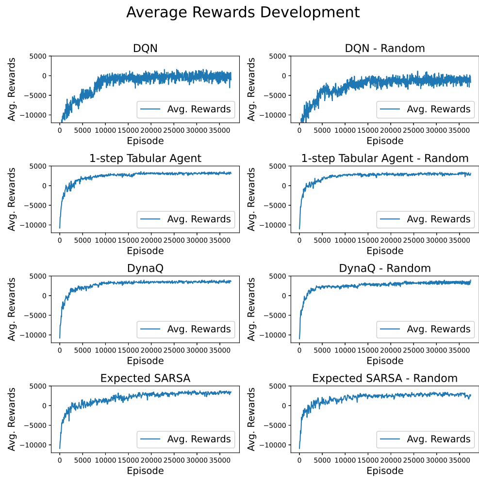
Figure 9. Comparison of average rewards development during training on random rewards for DQN and tabular agents
