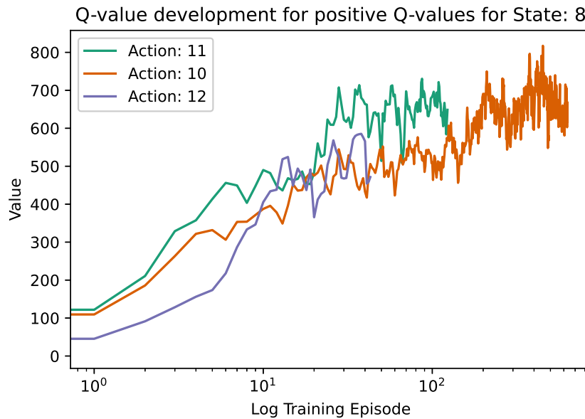
Figure 1. Q-value Trajectories for three potential decisions
