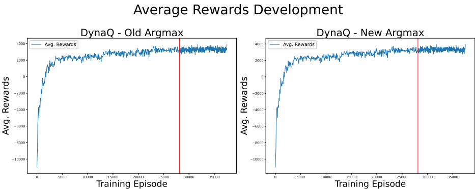
Figure 11. Comparison of average rewards during training for old and new argmax function for the DynaQ agent
