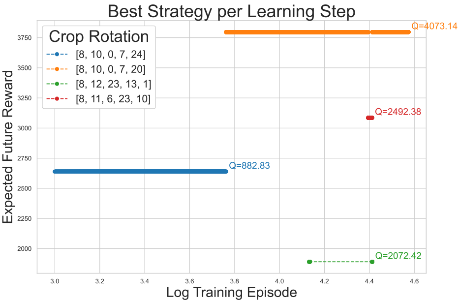
Figure 13. Chronological Development of the Best Strategy for Starting Crop 8 - Robust Learning
