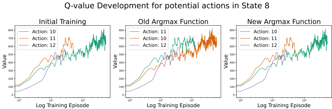
Figure 12. Q-value development comparison between old and new argmax function for 1 state-action pair
