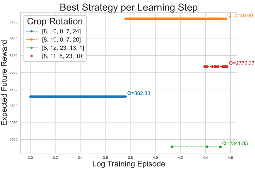
Figure 10. Chronological development of the best strategy for Starting Crop 8
