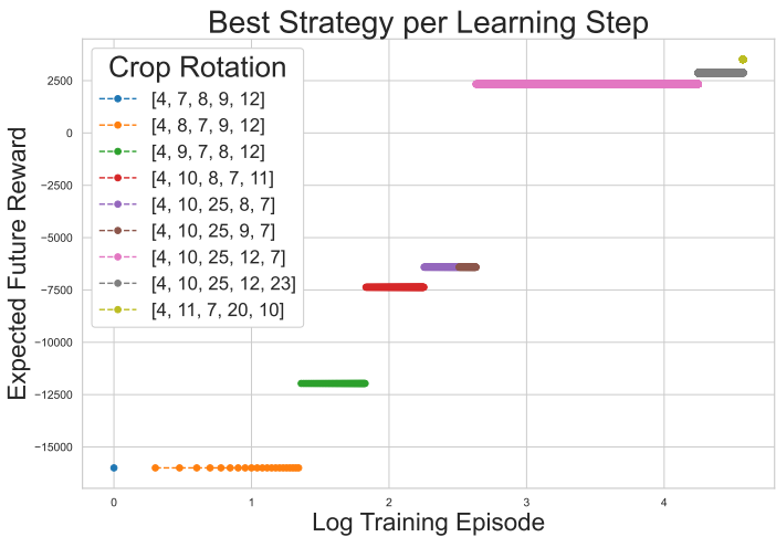
Figure 6. Chronological Development of the best Strategy for Starting Crop 4.
