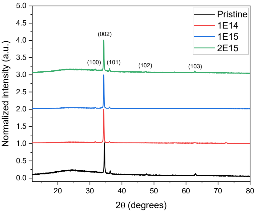
Figure 3. XRD Diffractograms of the irradiated and non-irradiated ZnO thin films.
