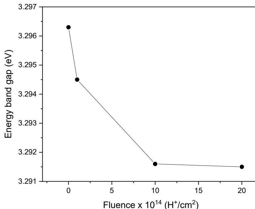
Figure 6. The energy band gap values of the pristine and irradiated ZnO samples.
