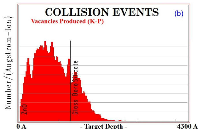
Figure 4. Comparison between defects created during 8 keV H^+ ions irradiation in ZnO, using fluences of (a) 1 \times 10^{14} H^+/cm^2 and (b) 2 \times 10^{15} H^+/cm^2 .
