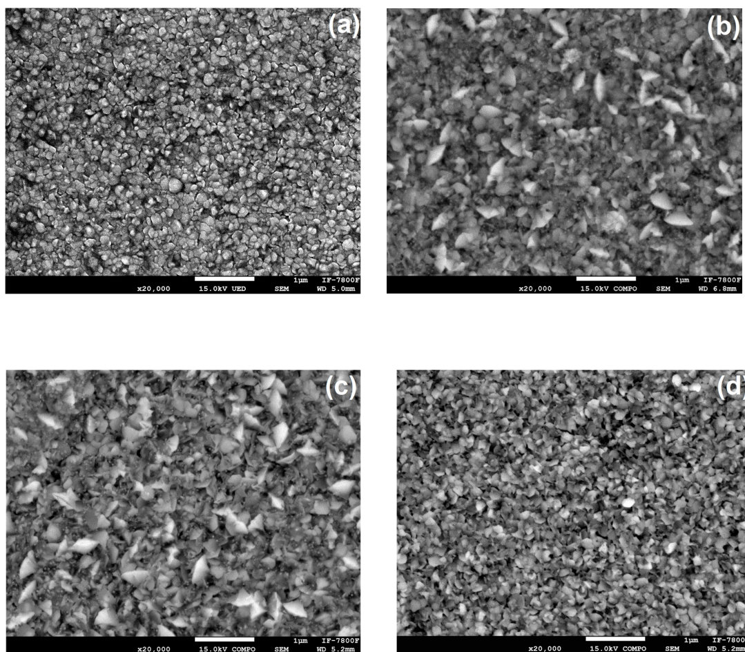
Figure 7. SEM micrographs of the (a) N-I, (b) 1E14, (c) 1E15, (d) 2E15 ZnO films.
