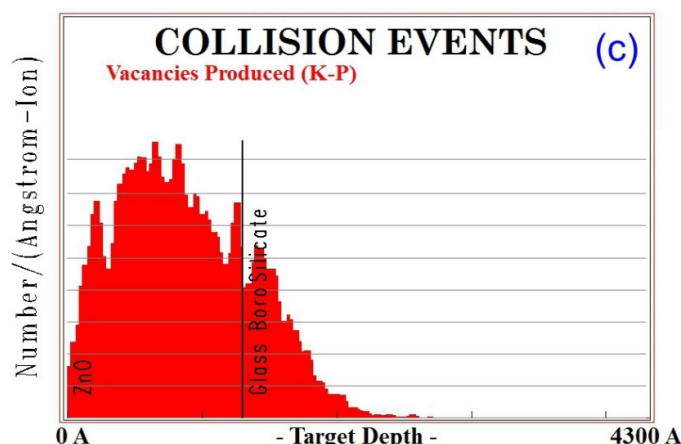
Figure 1. (a) Ion ranges, (b) ionization events, and (c) vacancies and defects produced during the irradiation of an 8 keV H^+ ion into a 116.18 nm ZnO thin film using a fluence of 2 \times 10^{15} H^+/cm^2 .
