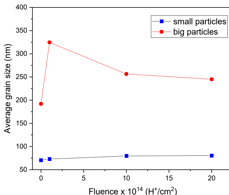
Figure 8. Dependence of average grain size with H^+ fluence.
