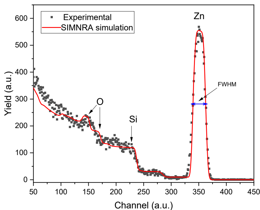
Figure 2. Experimental RBS (black dots) and simulated SIMNRA code (red line) spectra corresponding to the N-I ZnO thin film synthesized at 450 °C.
