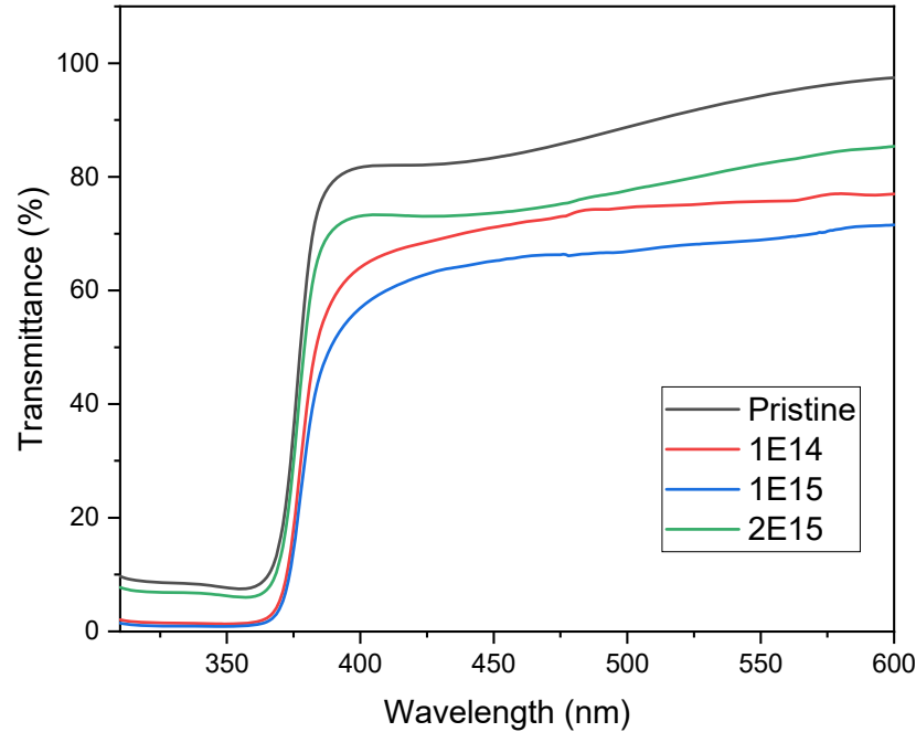
Figure 5. Optical transmittance spectra of the samples N-I (pristine), 1E14, 1E15 and 2E15.
