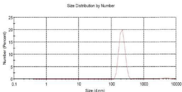
Figure 1. Size distribution of fucoxanthin nanoparticles by Dynamic Light Scattering.
