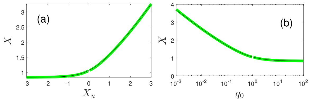
Figure 4. Approximate solution of transcendental equation. Exact numerical solution of Equation (133) (black) compared with the approximate solution (134)–(135) (green) versus (a) X_u and (b) q_0 .
