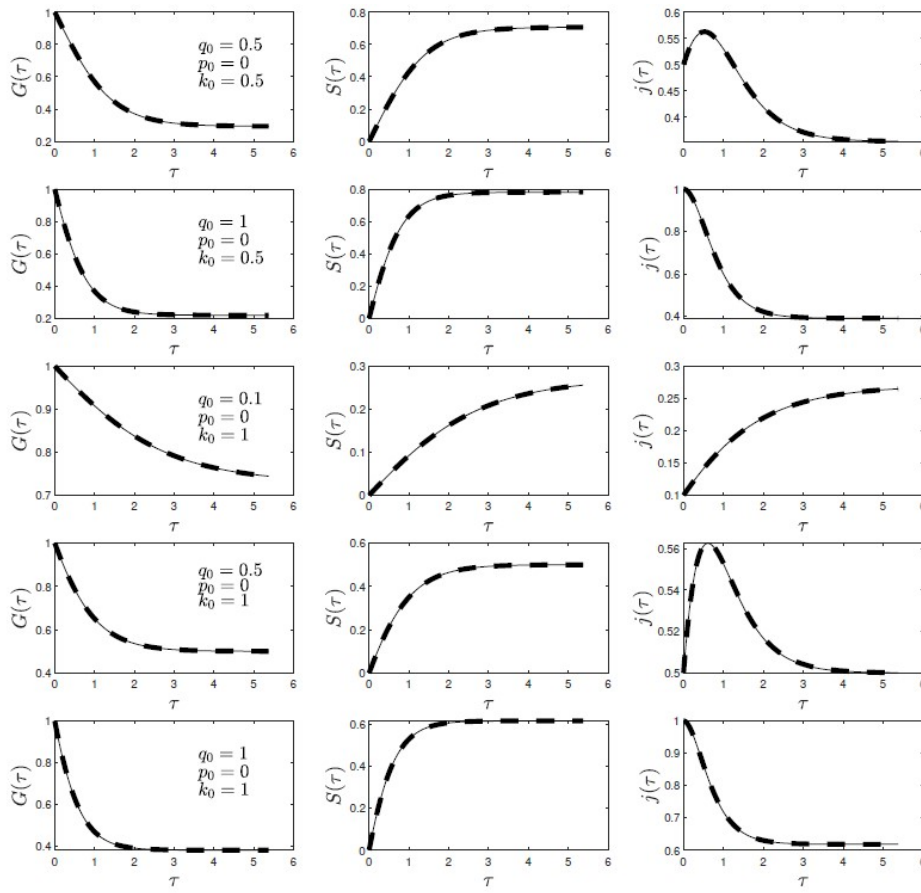
Figure 2. GS model. Numerical solution (thin solid line) and analytical solution, Equations. (32), (33), and (35) (thick dashed line) for the GS-limit with negligible stellar evolution ( p_0 = 0 ), and q_0, k_0 \in \{0.1, 0.5, 1.0\} . Shown are (left) G(\tau) , (middle) S(\tau) and (right) j(\tau) versus dimensionless \tau .
