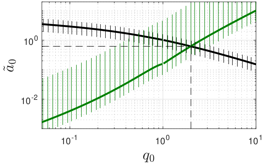
Figure 5. Observational constraint for GSL model parameters q_0 and \tilde{a}_0 . Equations (140) and (147) (black) and Equations (141) and (148) (green) for h_{70} = 1 . The vertical lines display the admissible ranges. The mean values cross at q_0 \approx 2.0 and \tilde{a}_0 \approx 0.622 (dashed). The green curve increases as q_0^{3/2} , while the black curve decreases as q_0^{-1} at q_0 \gg 1 , in agreement with Equations (152).
