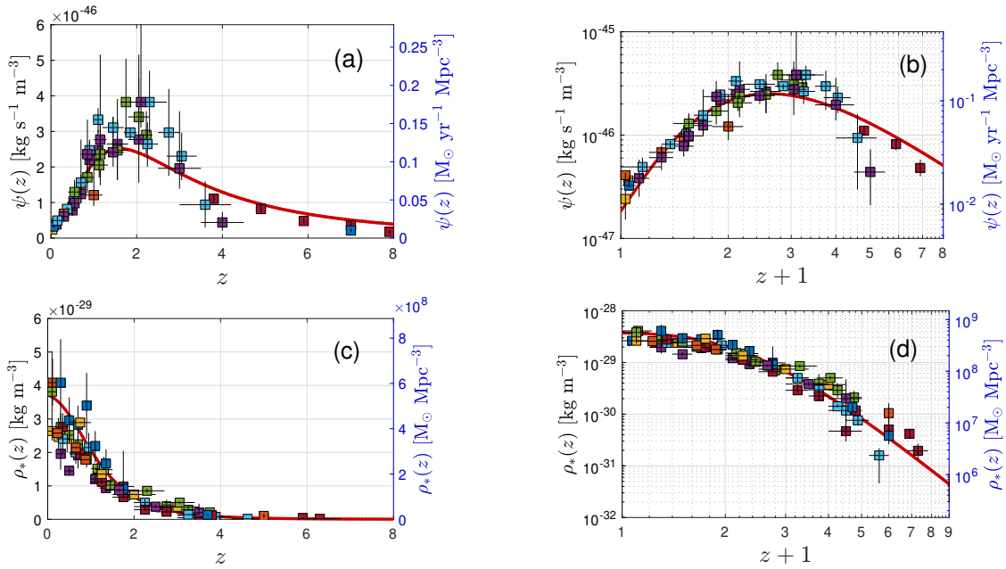
Figure 6. GSL model predictions. Fit to experimental data (symbols) from [7]. Our result (red solid line) for \tilde{a}_0 = 0.368 , q_0 = 2.97 , k_0 = 0.0039 , p_0 = 0.656 , i.e., k_0 + p_0 \approx 0.66 . Shown are both (a,b) \psi(z) and (c,d) \rho_*(z) in (a,c) linear and (b,d) double-logarithmic representations.
