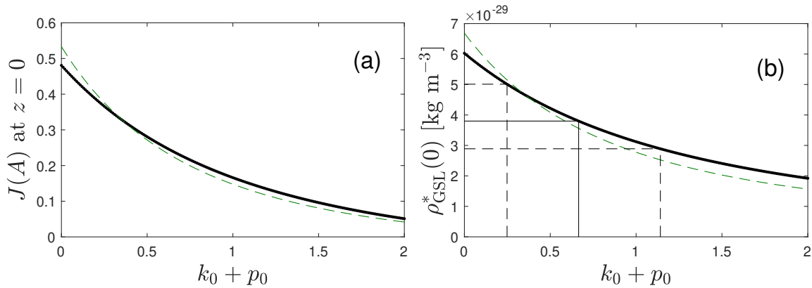
Figure 7. Observational constraint for GSL model parameter k_0 + p_0 . (a) Numerical J(A) from Equation (154) for z = 0 and (b) \rho_{\text{GSL}}^*(0) using this J(A) according to Equation (153), both versus k_0 + p_0 for q_0 = 2 , \tilde{a}_0 = 0.62 and h_{70} = 1 . The \rho_{\text{GSL}}^*(0) matches the value 3.80 \cdot 10^{-29} (127) at k_0 + p_0 \approx 0.66 (vertical solid line), in perfect agreement with our best fit to the experimental data (Figure 6). Taking into account experimental errors, the range of admissible k_0 + p_0 values is k_0 + p_0 \in [0.25, 1.14] (dashed vertical lines). The green dashed lines in panels (a) and (b) are the analytical expressions (159) and (160).
