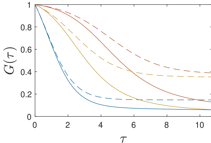
Figure 3. GSL model. Fraction G_s(\tau) (dashed) compared with the numerically calculated G(\tau) (solid) for several choices of the parameters p_0 , k_0 , and q_0 : (blue) k_0 = 0.1 , p_0 = 0.1 , q_0 = 0.3 , (red) k_0 = 0.02 , p_0 = 0.37 , q_0 = 0.02 , and (yellow) k_0 = 0.02 , p_0 = 0.37 , q_0 = 0.07 . The numerical G(\tau) approaches zero in the limit \tau \rightarrow \infty , while the small time approximation G_s(\tau) remains finite.
