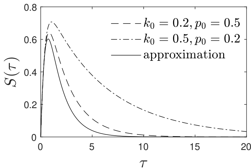
Figure 9. Feature of the approximate GSL solution. S(\tau) versus \tau according to Equations (105), (107), and (110) for q_0 = 2 and two cases for which the sum k_0 + p_0 is identical. The analytical approximation yields just one curve (solid), while the numerical solutions (dashed and dot-dashed) of the GSL-equation differ.
