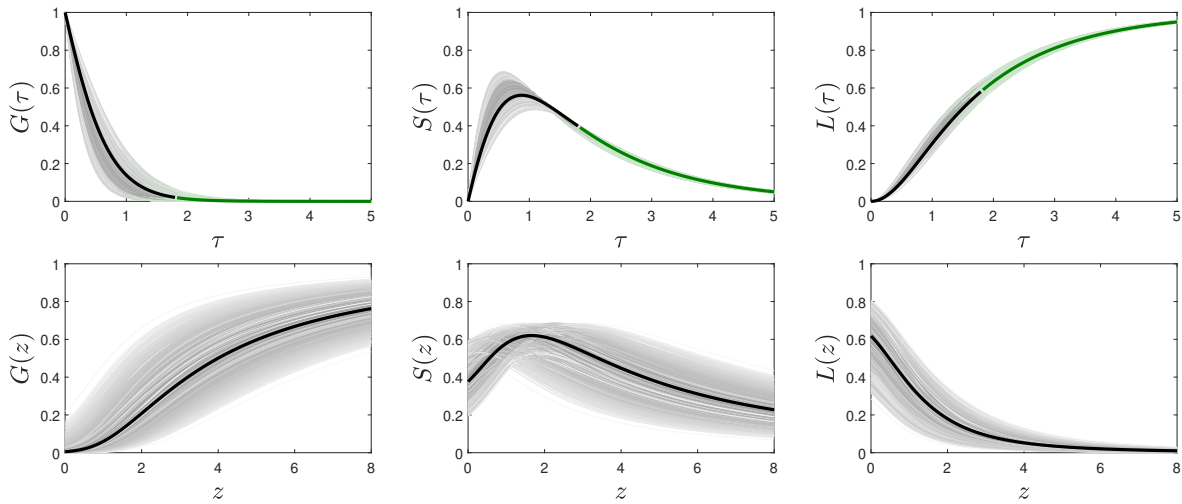
Figure 8. GSL model predictions. G , S , and L for the parameters \tilde{a}_0 = 0.62 , q_0 = 2 , k_0 = 0.0039 , p_0 = 0.656 . The lines in (a) are G(\tau) (106), S(\tau) (110), and L(\tau) = 1 - G(\tau) - S(\tau) (120) obtained using the approximation Equation (69) for U(\tau) = -\ln[Y(\tau)] with coefficients c_1 , \alpha_1 , and \alpha_2 given by Equation (105). Lines in (b) are G(z) = G(\tau(z)) etc. with \tau(z) from Equation (10). Error bars from Equation (149). They are represented as gray lines, whose darkness moderately increases with their probability, assuming Gaussian distributed \tilde{a}_0 and q_0 . The future corresponding to \tau \geq \tau(0) = 5.37\tilde{a}_0\sqrt{3} \approx 1.83 , is colored green. Note that the error bars in panel (a) are smaller than in panel (b) because the fractions (106), (110), (120) as a function of reduced time only depend on the parameter q_0 but not on the parameter \tilde{a}_0 .
