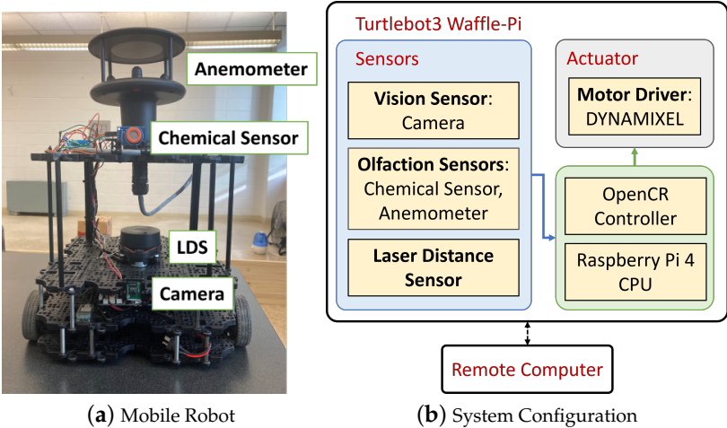
Figure 7. (a) Turtlebot3 platform based mobile robot is used in this work. In addition to the built-in camera and Laser Distance Sensor, the robot is equipped with a chemical sensor and an anemometer for measuring chemical concentration, wind speeds, and airflow directions. (b) System configuration consisting of the robot platform and a remote PC. The solid line indicates a physical connection, while the dotted line represents a wireless link.
