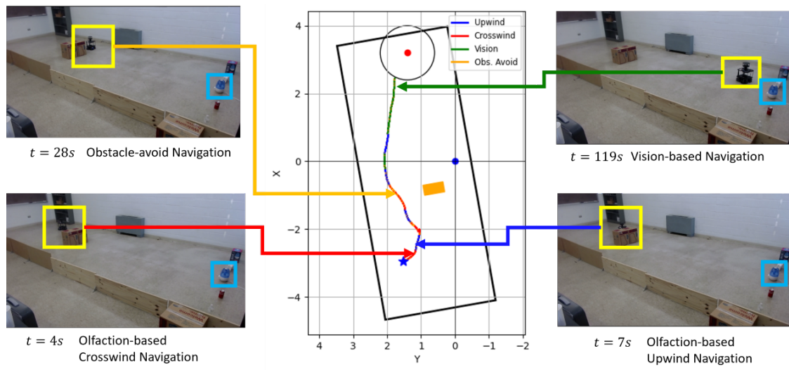
Figure 8. Trajectory graph of a successful sample run with the proposed multi-modal LLM-based OSL algorithm in laminar airflow environment. The navigation behaviors are color-separated. The obstacle is indicated by orange box, and the odor source is represented by a red point with the surrounding circular source declaration region.
