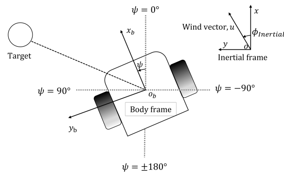
Figure 3. Robot notations. Robot position (x, y) and heading \psi are monitored by the built-in localization system. Wind speed u and wind direction are measured from the additional anemometer in the body frame. Wind direction in inertial frame \phi_{Inertial} is derived from robot heading \psi and wind direction in body frame.
