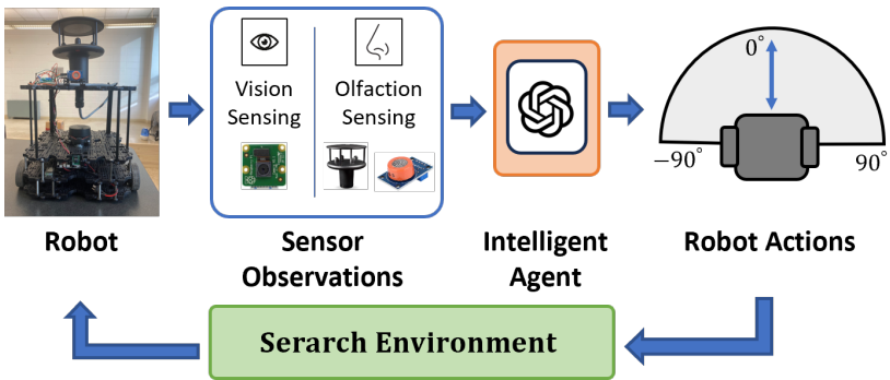
Figure 1. Flow diagram of the proposed method for the OSL experiment. We utilized the Turtlebot3 robot platform. We equipped it with a camera, Laser Distance Sensor, airflow sensor, chemical sensor, etc. The proposed algorithm utilizes multi-modal LLM for navigation decision-making.
