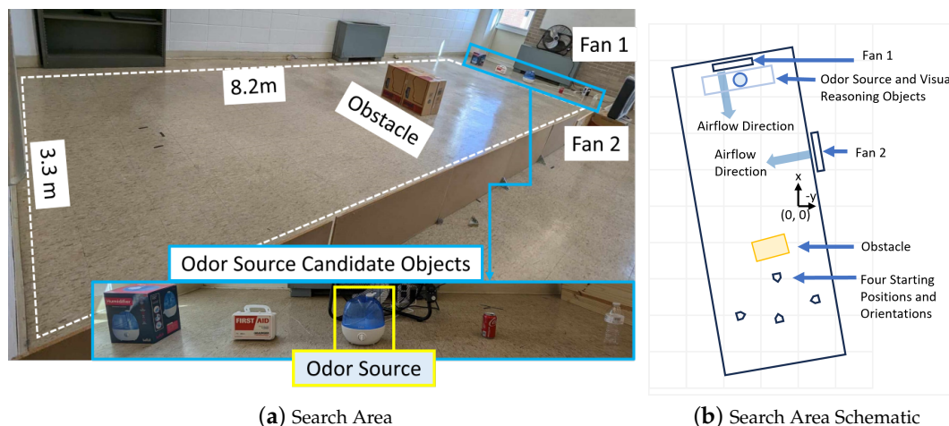
Figure 6. (a) The experimental setup. The robot is initially placed in a downwind area with the objective of finding the odor source. A humidifier loaded with ethanol is employed to generate odor plumes. Two electric fans are placed perpendicularly to create artificial wind fields. An obstacle is placed in the search area. There are 5 objects to test the reasoning capability of the LLM-model. (b) Schematic diagram of the search area. The four robot starting positions are used for testing the performance of the proposed OSL algorithm.
