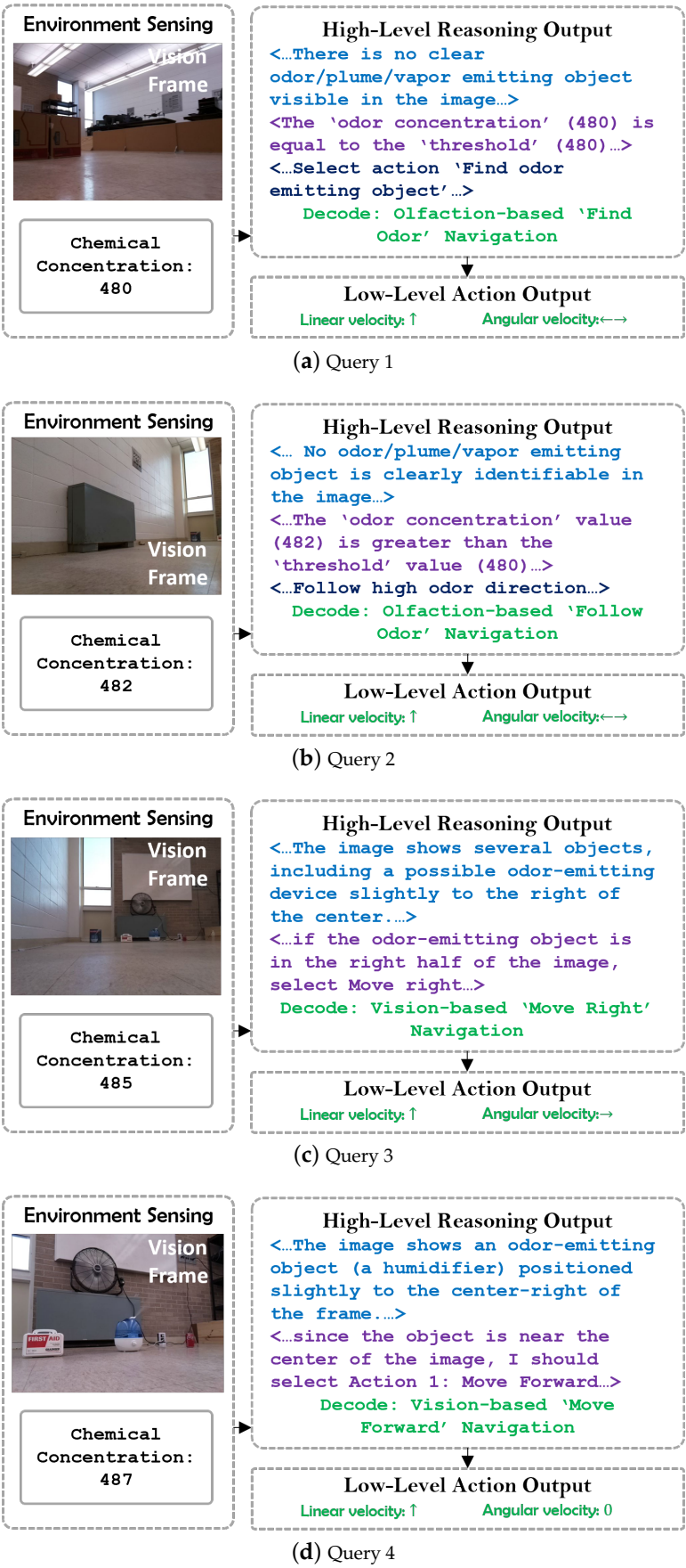
Figure 9. Examples of 'Environment Sensing' and 'Reasoning Output' by the GPT-4o model.
