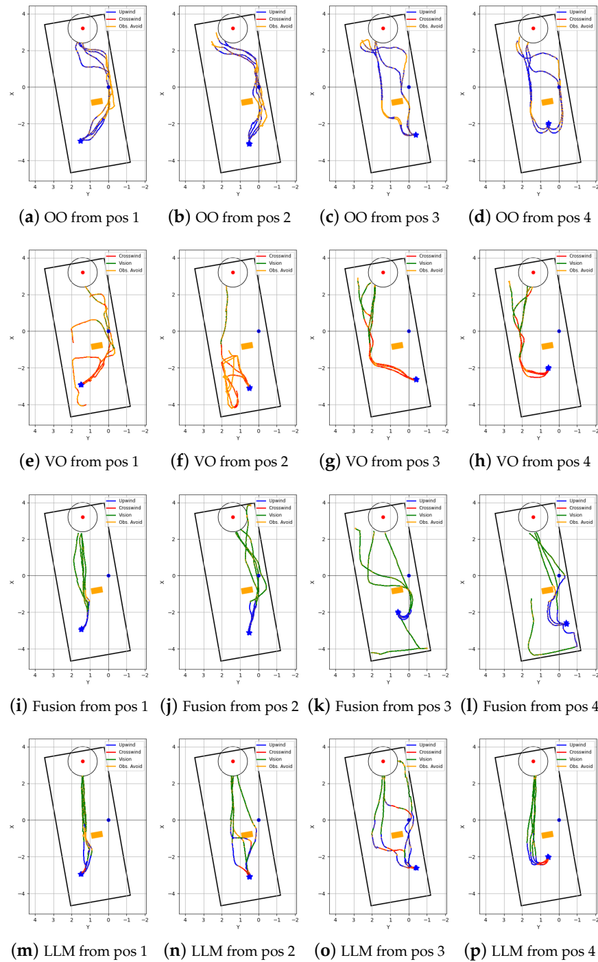
Figure 10. Robot trajectories of repeated tests in laminar airflow environment: (a–d) ‘Olfaction-only’ (OO); (e–h) ‘Vision-only’ (VO); (i–l) ‘Vision and Olfaction Fusion’ (Fusion); and (m–p) ‘LLM-based’ (LLM) navigation algorithms.
