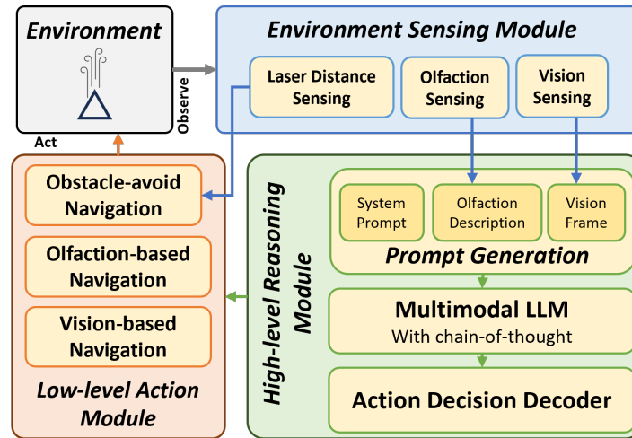
Figure 2. The framework of the proposed multi-modal LLM-based navigation algorithm. The three main modules are the 'Environment Sensing Module', 'High-level Reasoning Module', and 'Low-level Action Module'.
