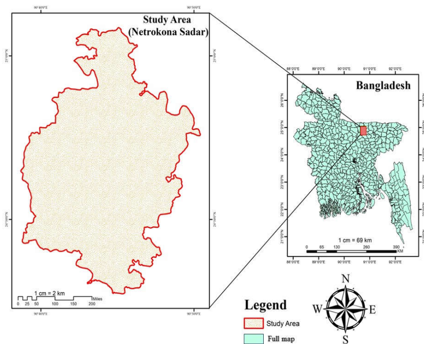
Figure 2. : Study Area (Netrokona Sadar).
