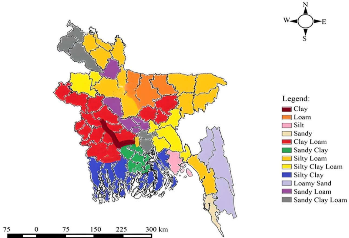
Figure 4. Soil classification Map of study area [Netrokona Sadar]( Islam et al., 2017).
