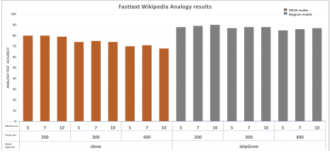
(f) Fasttext models analogy test results For Wiki corpus
