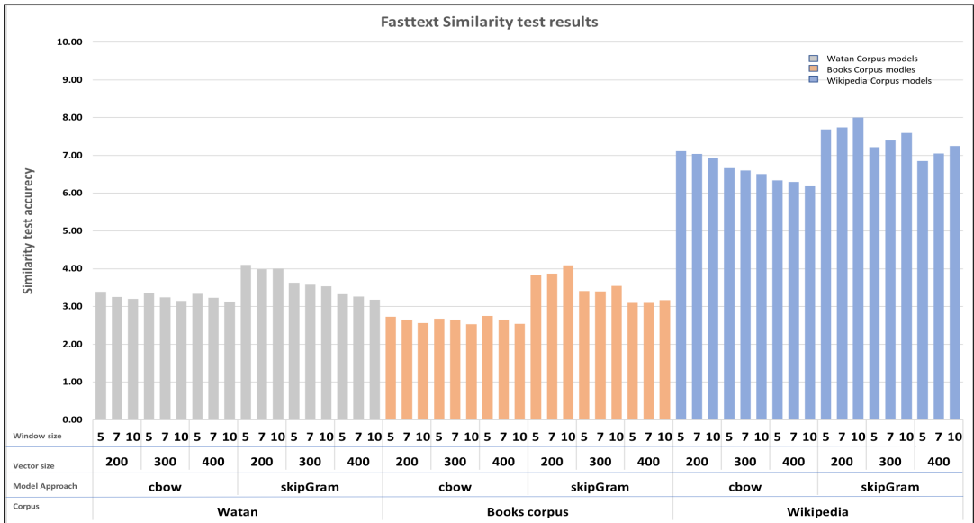
Figure 12. Fasttext models similarity test results.
