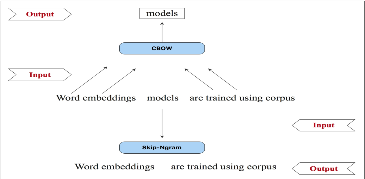
Figure 1. Illustration of the Skip-gram and Continuous Bag-of-Words (CBOW) models.
