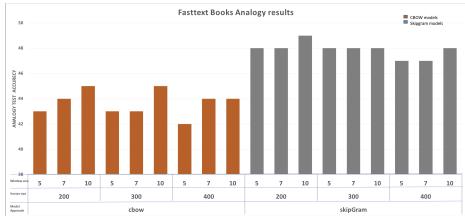
(d) Fasttext models analogy test results For Books corpus
