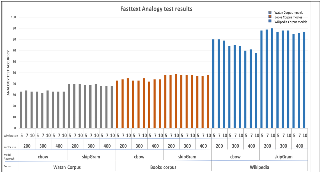
Figure 7. Fasttext models analogy test results.
