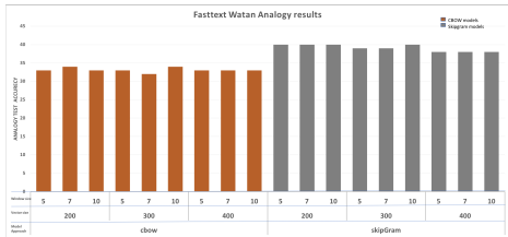
(b) Fasttext models analogy test results For Watan corpus
