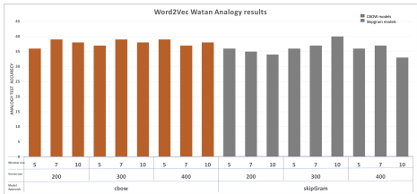
(a) Word2Vec models analogy test results For Watan corpus
