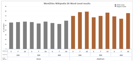
(e) Word2Vec models SA results For Wiki corpus
