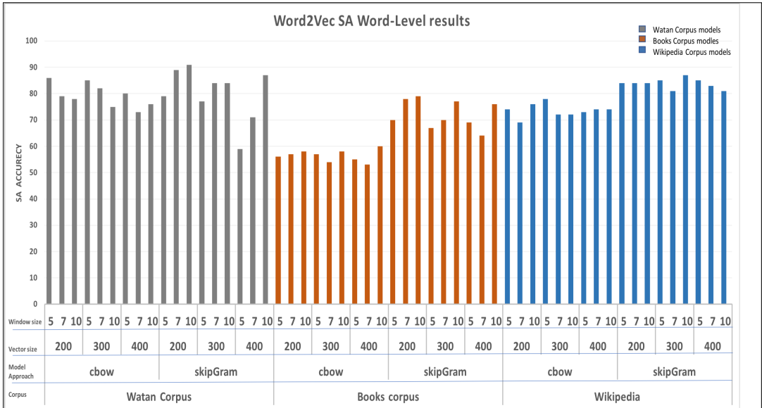
Figure 8. Word2Vec models Sentiment analysis results.
