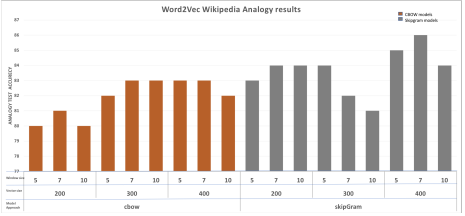
(e) Word2Vec models analogy test results For Wiki corpus
