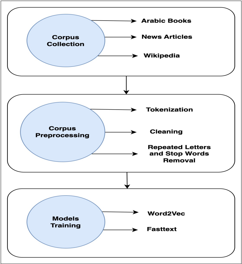
Figure 2. Building Arabic Word Embeddings Methodology.
