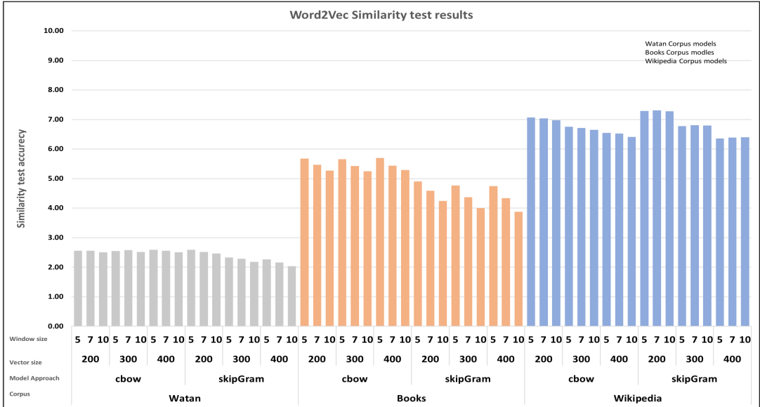
Figure 11. Word2Vec models similarity test results.
