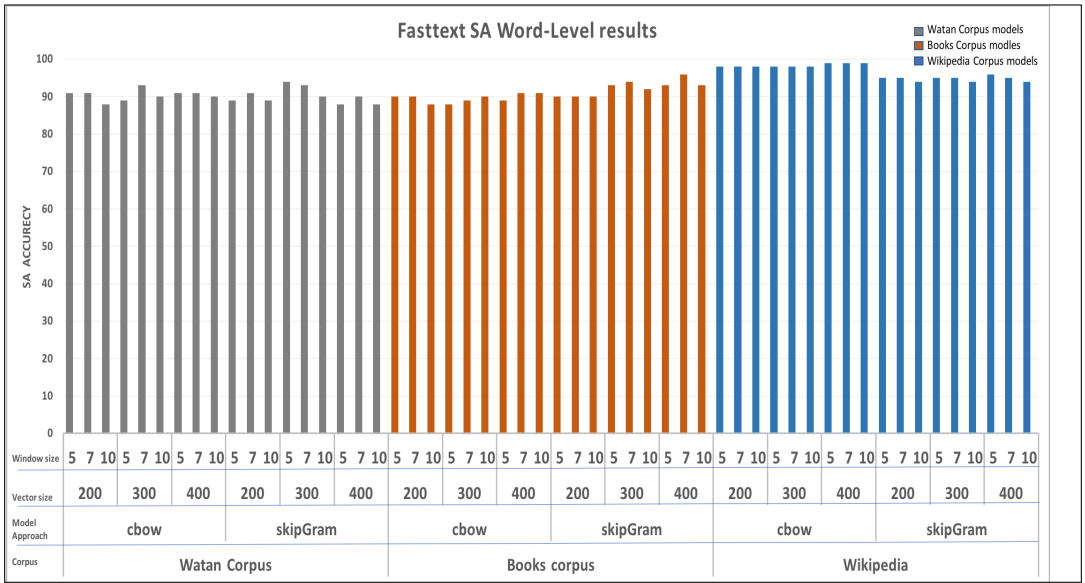
Figure 9. Fasttext models Sentiment analysis results.
