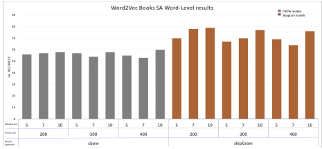
(c) Word2Vec models SA results For Book corpus
