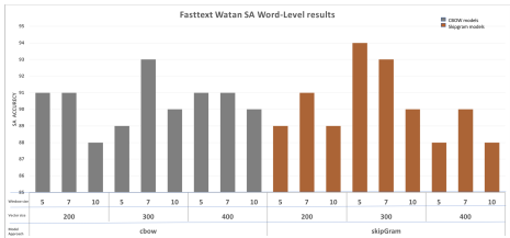
(b) Fasttext models SA results For Watan corpus
