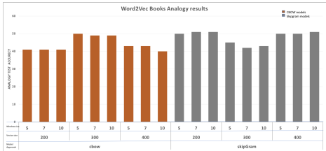
(c) Word2Vec models analogy test results For Book corpus
