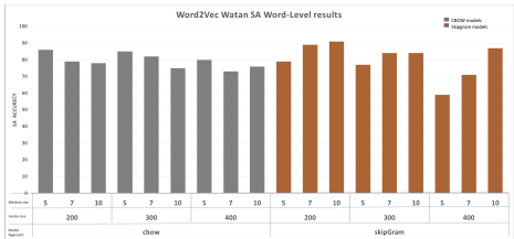
(a) Word2Vec models SA results For Watan corpus
