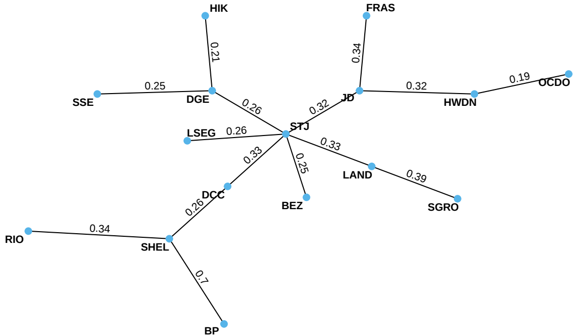
Tree 1
