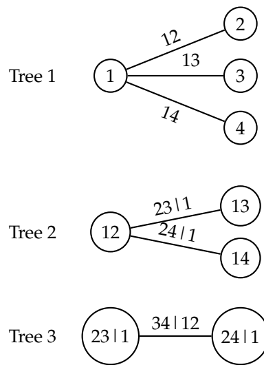
Figure 1. Example of C-Vine structures for d = 4 .
