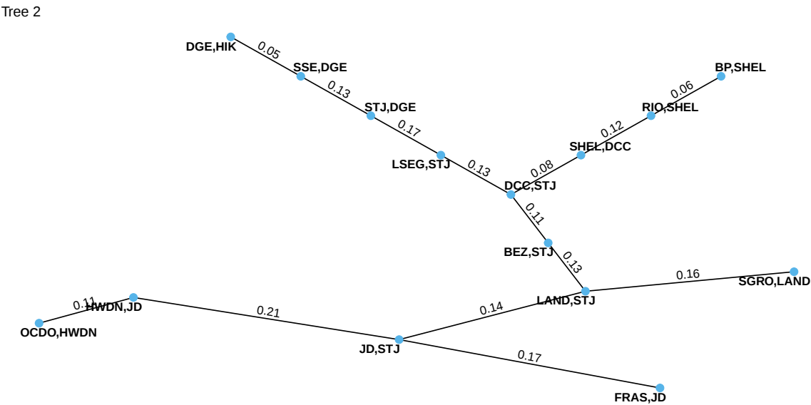
Figure 5. The second tree structure of estimated R-Vine and Kendall’s tau values for each connected pair of stocks.
