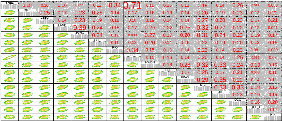
Figure 3. Pairwise normalized contour plots.
