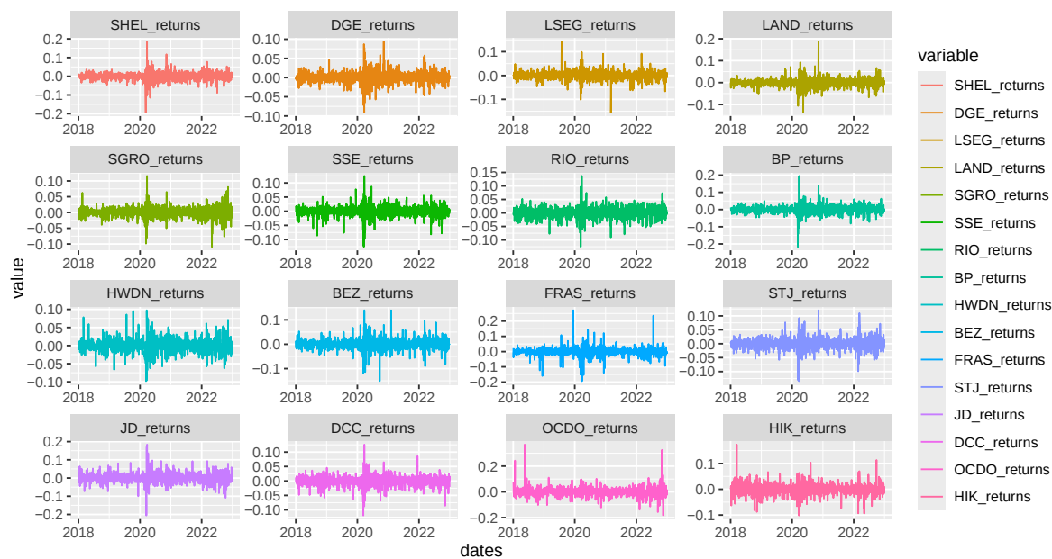
Figure 2. Daily log-returns.
