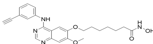
Figure 7. Molecular structure of CUDC-101.
