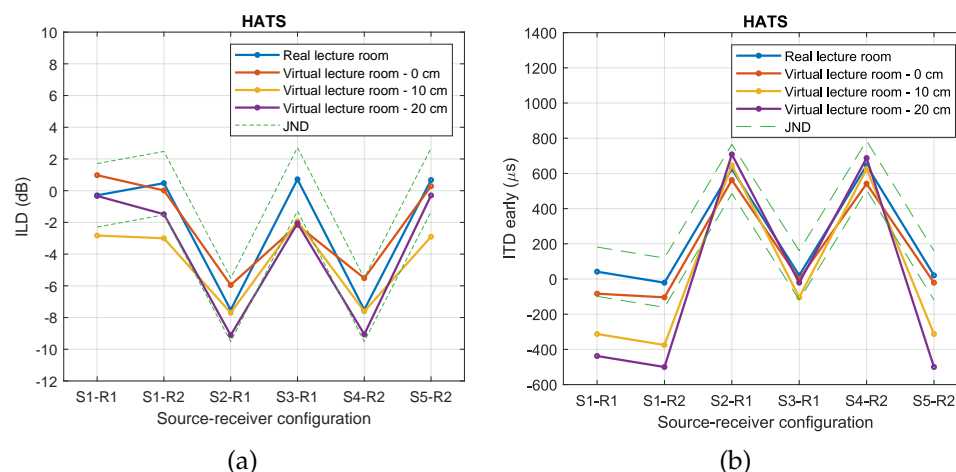
Figure 17. Values computed for the real and virtual lecture rooms for different off-center positions of the HATS within the ASL as a function of the source-receiver configuration for: (a) ILD band-passed from 1 to 9 kHz; (b) early ITD band-passed from 100 to 9000 Hz.
