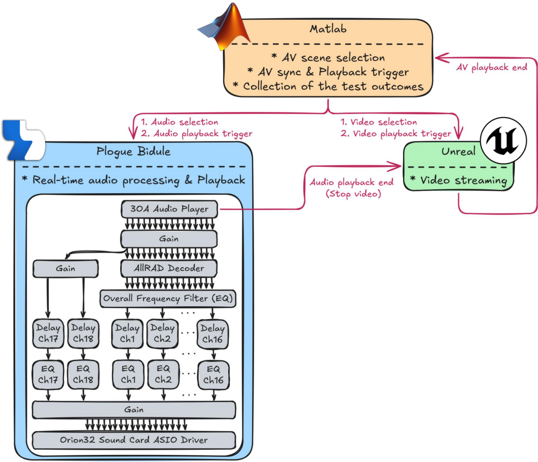
Figure 3. Scheme of the software framework components and their interconnections at the basis of the proposed VR system.
