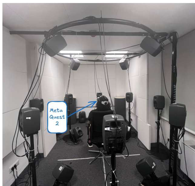
Figure 4. Picture of the VR system inside the ASL during the execution of a speech intelligibility test on a listener.
