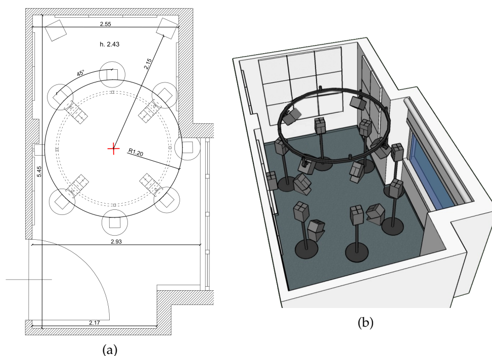
Figure 1. (a) ASL floor plan with the projected VAE reproduction system. The red cross marks the listening position. (b) 3D model of the ASL with spherical 16-speaker array.
