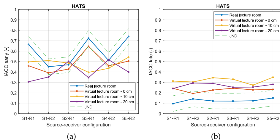
Figure 18. Values computed for the real and virtual lecture rooms for different off-center positions of the HATS within the ASL as a function of the source-receiver configuration for: (a) early IACC averaged across the 500 to 2000 Hz octave bands; (b) late IACC averaged across the 500 to 2000 Hz octave bands.
