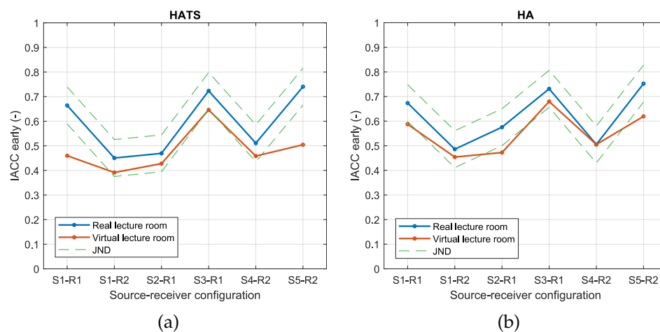
Figure 15. Early IACC values averaged across the 500 to 2000 Hz octave bands and JND limits for the real and virtual lecture rooms as the source-receiver configuration varies, for measurements with: (a) the HATS; (b) the HA.
