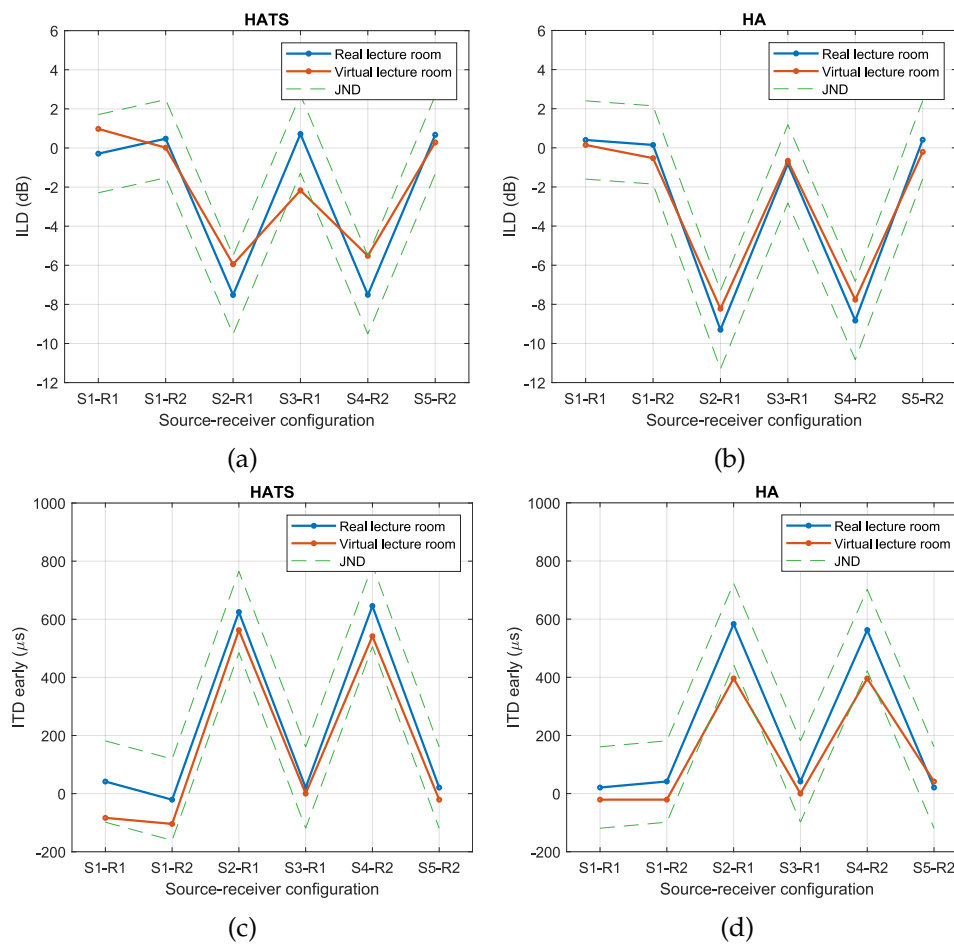
Figure 14. ILD values, pass-banded from 1 to 9 kHz, for the real and the virtual lecture room and JND limits as the source-receiver configuration varies, for measurements with: (a) HATS; (b) HA. Early ITD values, pass-banded from 100 to 1400 kHz, for the real and the virtual lecture room and JND limits as the source-receiver configuration varies, for measurements with: (c) HATS; (d) HA.
