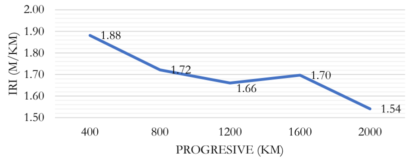
Figure 6. IRI left lane Merlin roughness tester.
