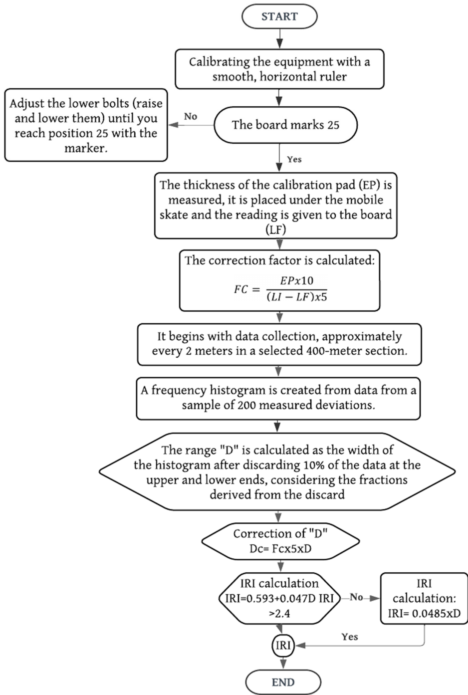
Figure 1. Flowchart of the Rugosimeter Merlin Equipment method.
