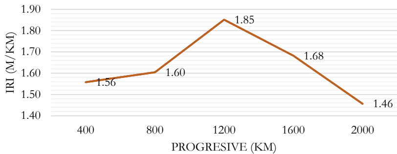
Figure 5. IRI right lane Merlin roughness tester.
