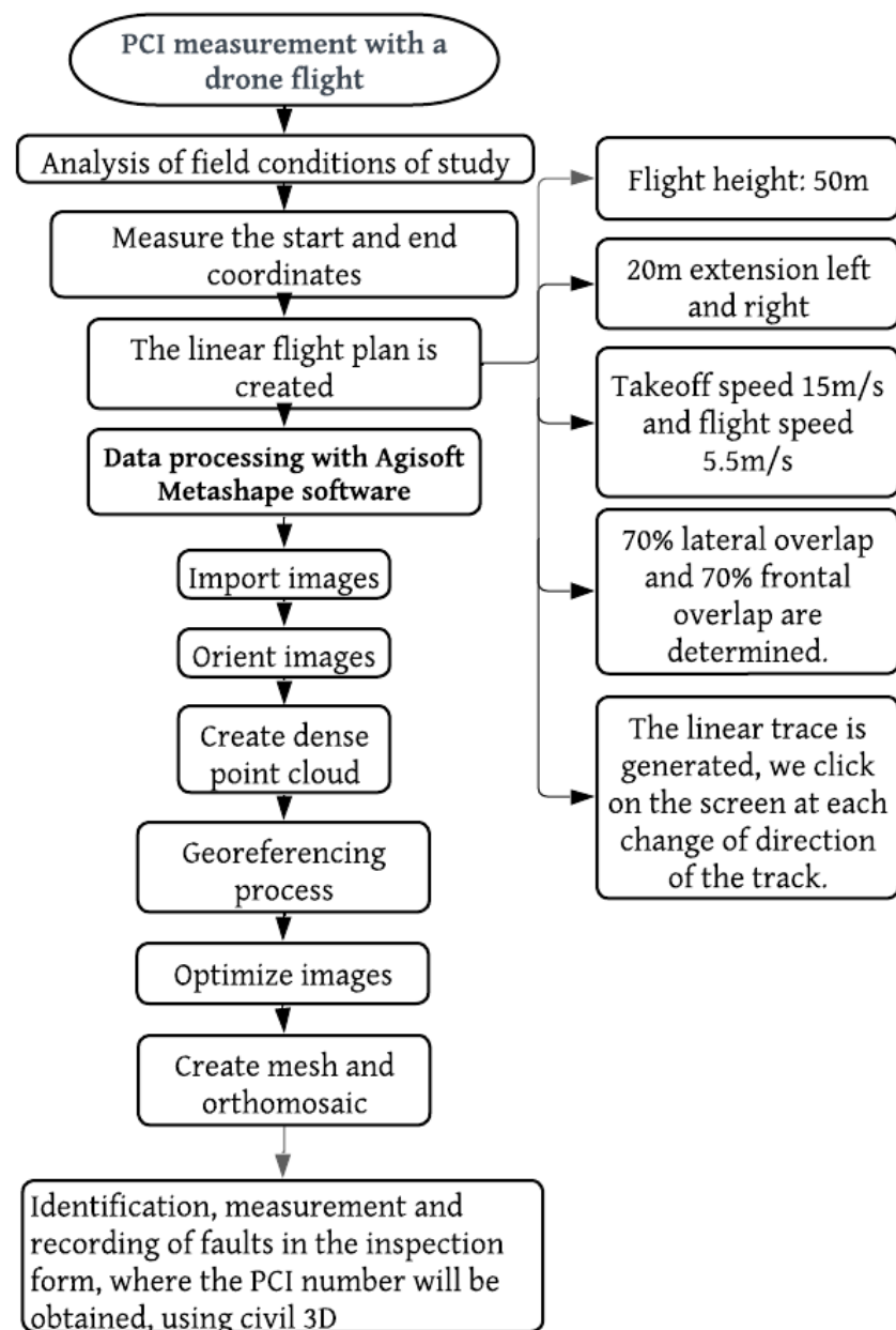
Figure 4. PCI evaluation by flying the DJI Mavic 2 pro Drone.
