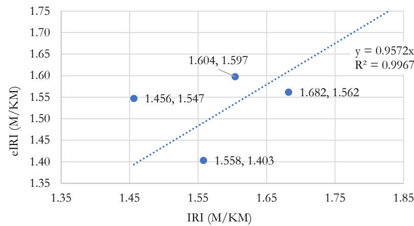
Figure 9. IRI vs eIRI dispersion table—Right Lane.
