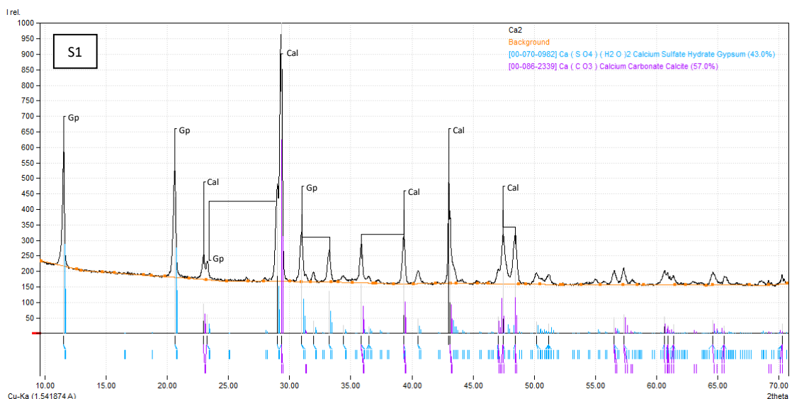
Figure S.- DRX pattern of samples in the DAS-Ca: S1 (Ca2, 7.5 cm); S2 (Ca3, 8.5 cm); S3 (Ca4, 10 cm); S4 (Ca5, 15 cm) and DAS-Mg: S5 (Mg2, 12 cm), as well as S6 (Pindo, drain-sand of the bottom columns), showing the main mineral phases identified* and their correlation with the patterns obtained from database by Match. Mineral symbol according to IMA–CNMNC (Warr, 2021). * Semiquantitative results have been improved by Rietveld refinement (See Table 3).
