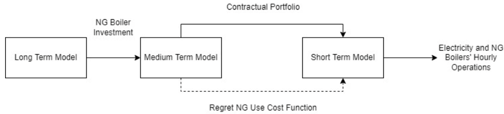
Figure 1: LC decision problem by analysis horizon.
