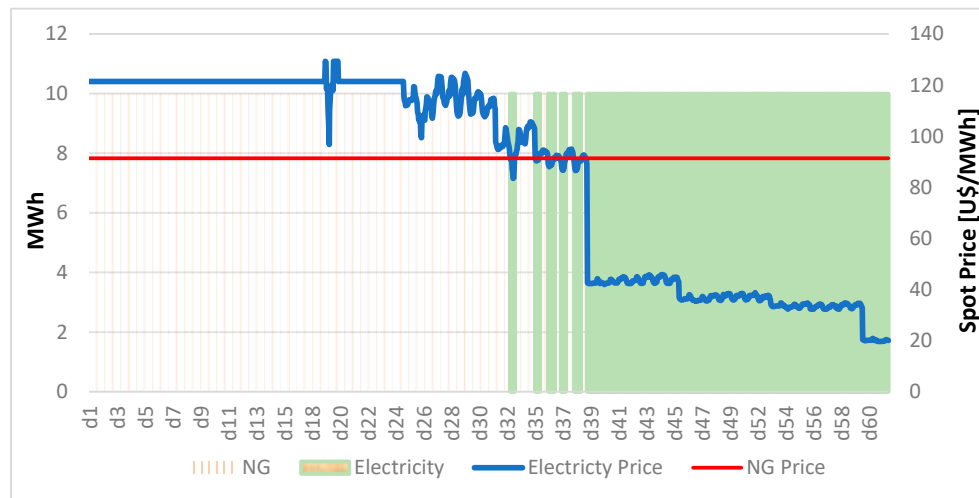
Figure 7. NG and electricity consumption × NG and electricity prices for simulation beginning in IM3.
