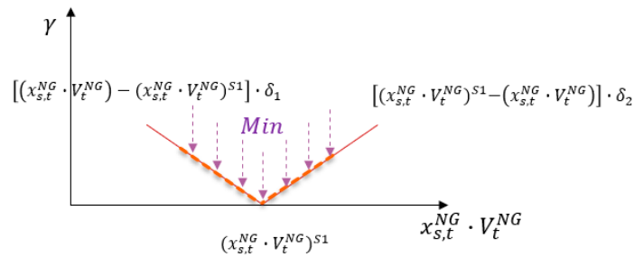
Figure 3. Construction methodology of the regret cost function.
