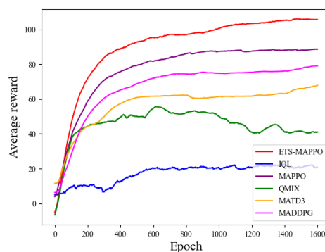
Figure 8. Comparison of the average reward values of the six algorithms.
