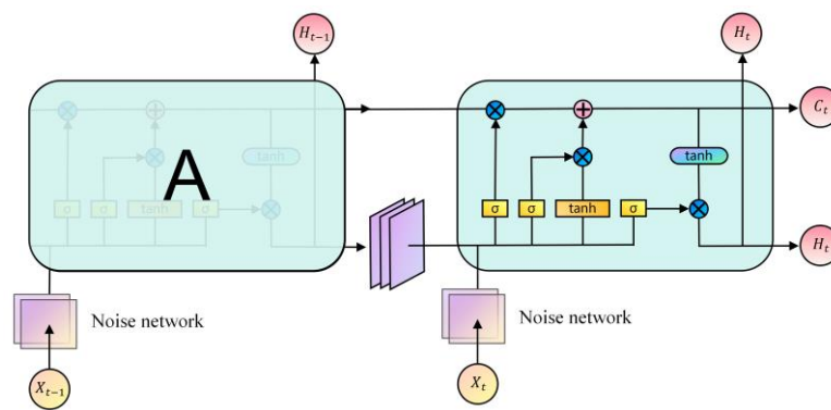
Figure 4. The STEE network architecture.
