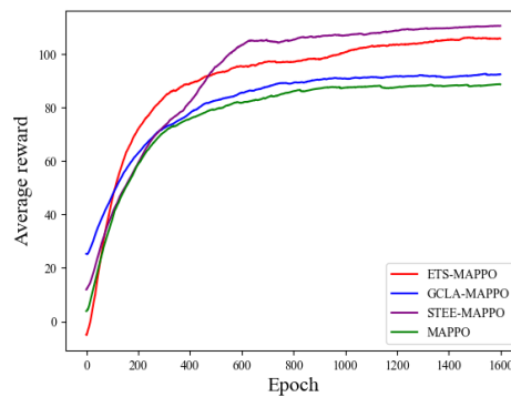
Figure 11. Comparison of average reward results from ablation experiment.
