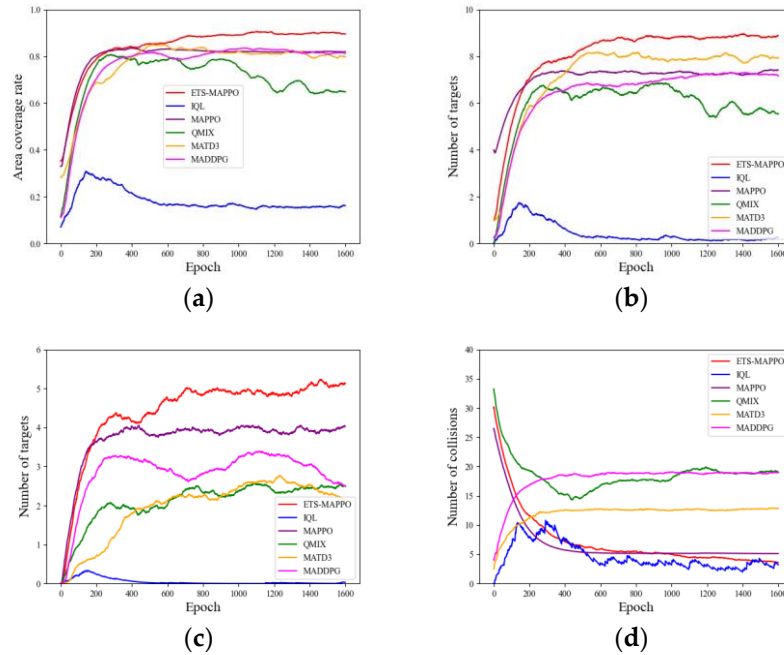
Figure 9. The specific parameter metrics train results. (a) Area coverage rate, (b) The number of initial target searches; (c) The number of target re-searches; (d) The number of collisions.
