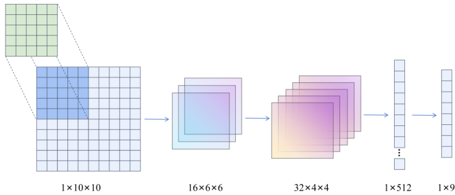
Figure 6. Processing of TEPM convolutional operations for 10 \times 10 state parameters.
