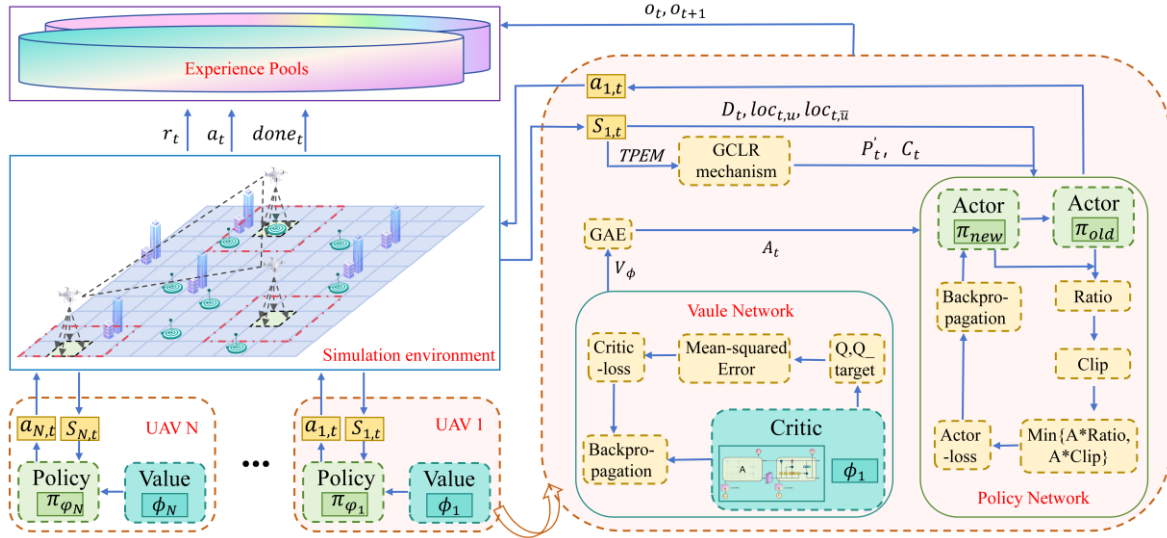
Figure 7. The ETS-MAPPO algorithmic framework.
