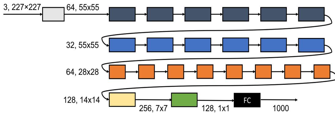
Figure 3. SqueezeNext network architecture (23 layers) [49].
