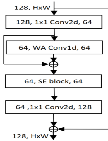
(b) Residual 1D CNNs block with SE layer (SEC) [52].
