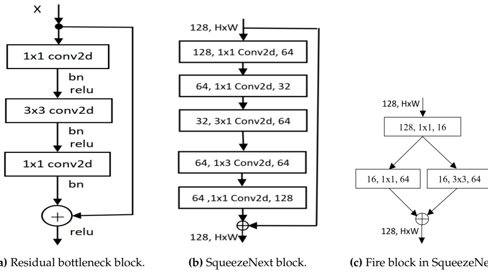
Figure 1. Illustration of (a) ResNet bottleneck block [48], (b) SqueezeNext block [49], and (c) SqueezeNet file module [50].
