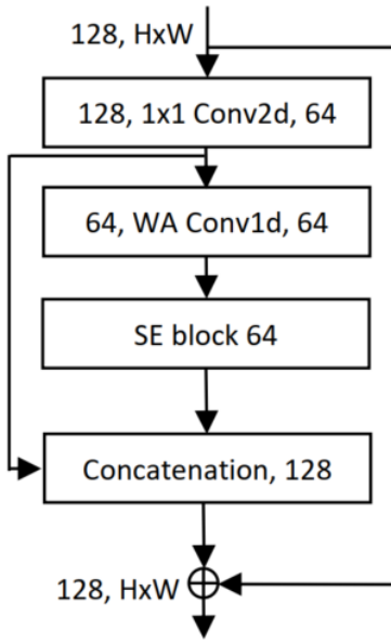
(c) Reduced CNN layers block [54,55].
