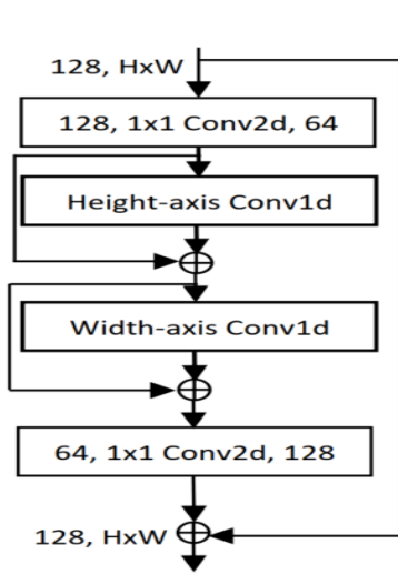
(a) Residual 1D CNNs block [51].
