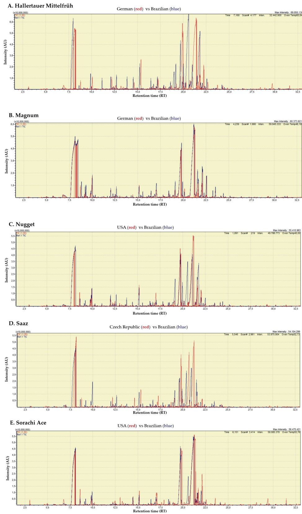
Figure 1. Chemical interpretation of the PLS-DA model discriminating between hops planted in their countries of origin (red) and the same varieties planted in Brazil (blue). Samples are based on VIP
