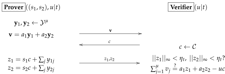
Figure 3. The JAK ID Scheme
