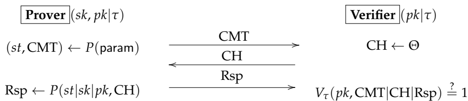
Figure 1. Canonical Identification Protocol.
