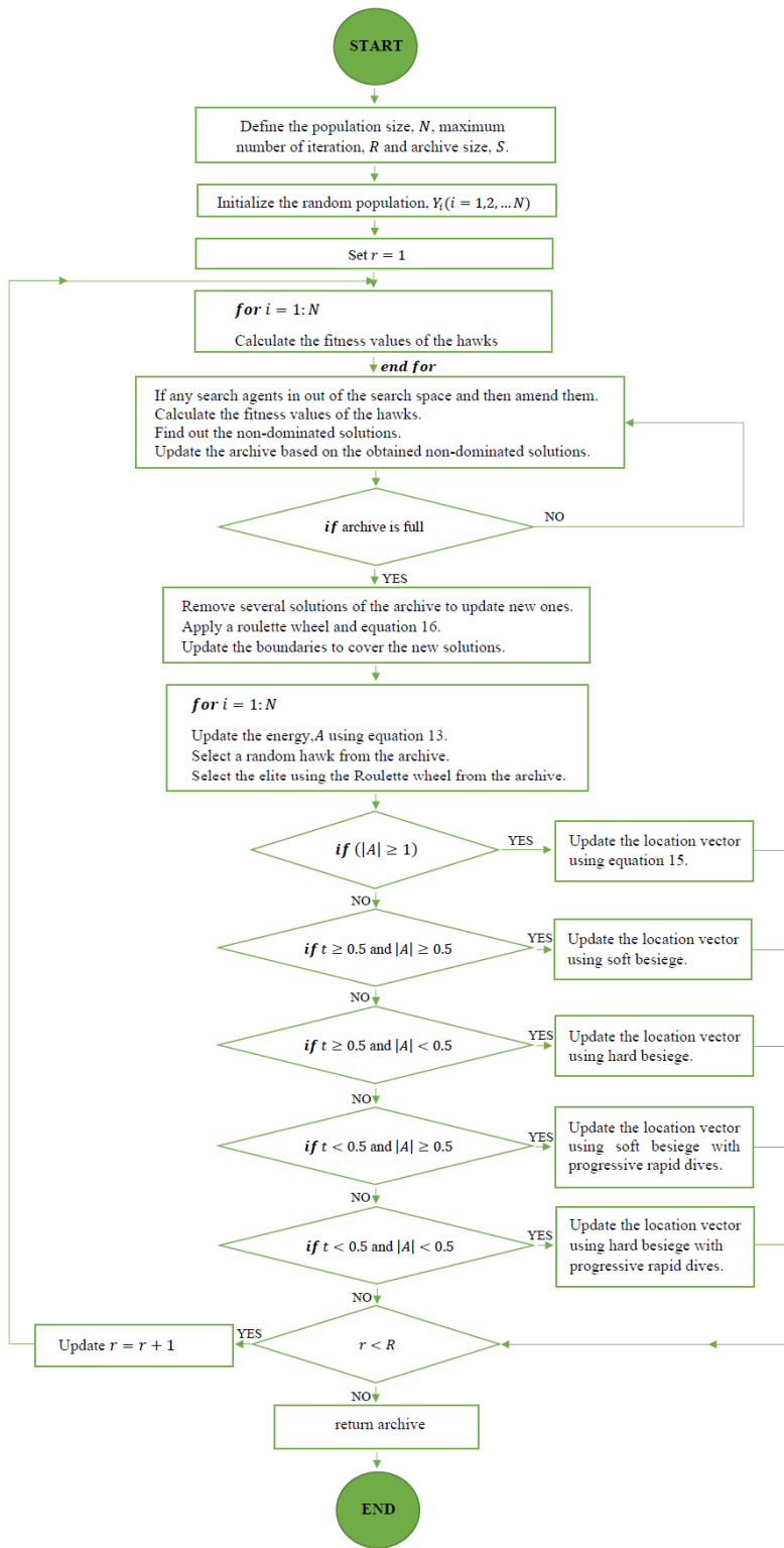
Figure 3. Flowchart for multi-objective harris hawk optimization.
