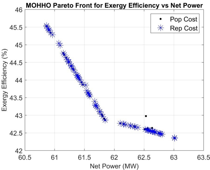
Figure 7. Pareto front showing the trade-off between exergy efficiency and net power.
