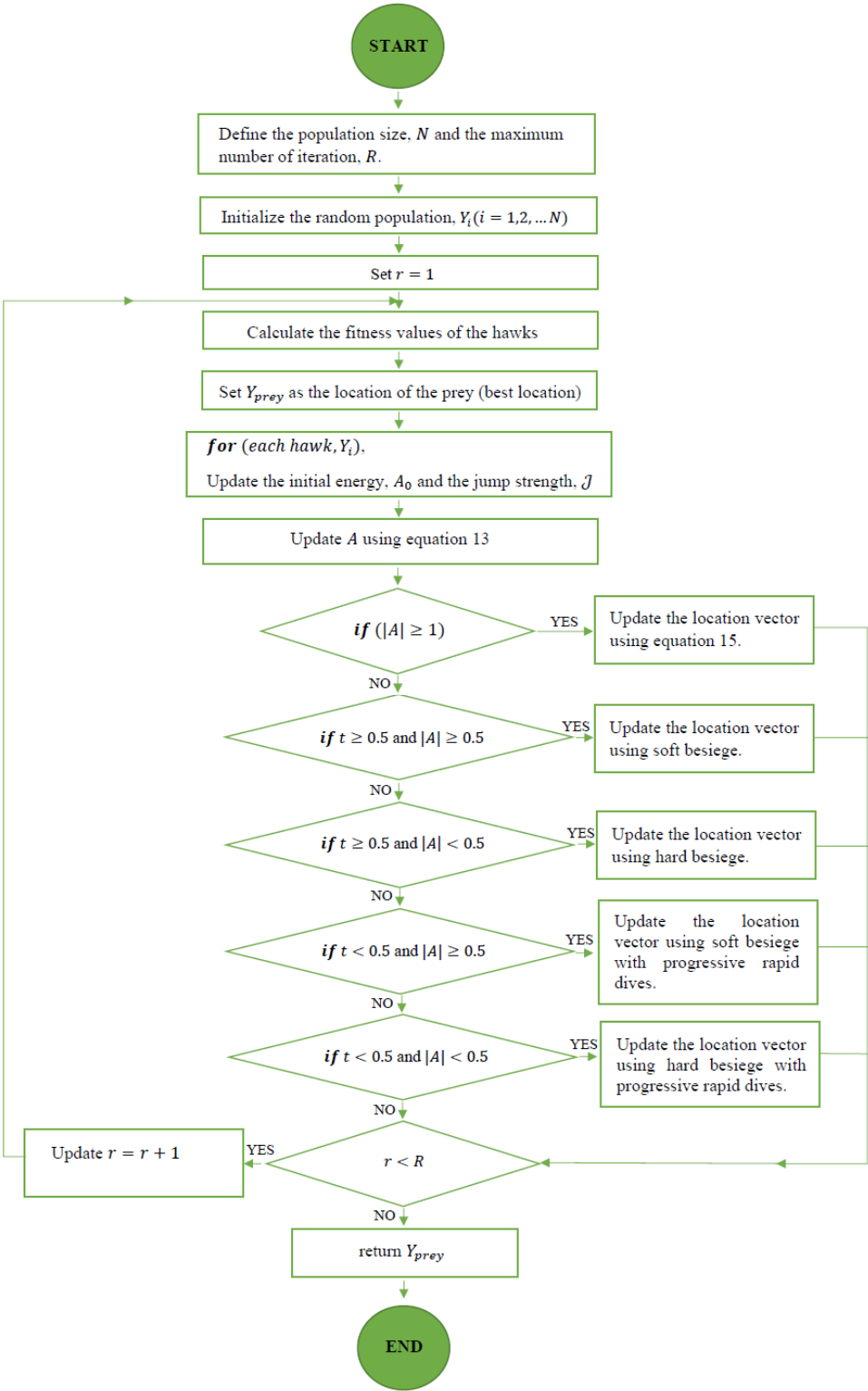
Figure 2. Flowchart for single-objective harris hawk optimization.
