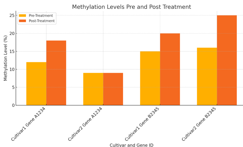
Figure 4. Methylation Levels and Pre and Post Treatment.
