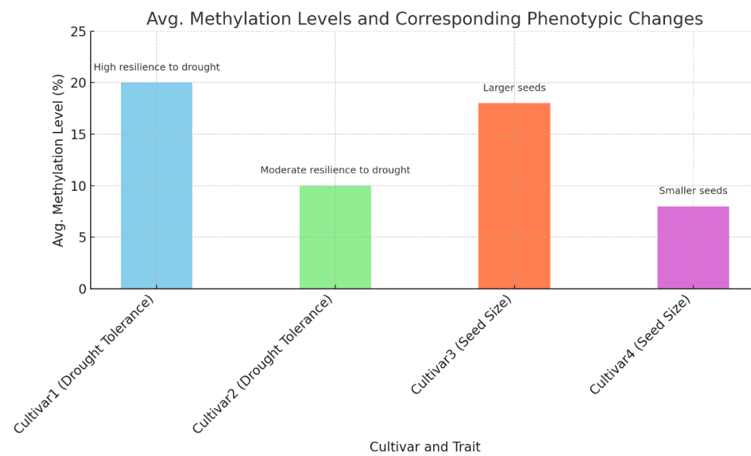
Figure 6. Averages of Methylation Levels and Corresponding Phenotypic Changes.
