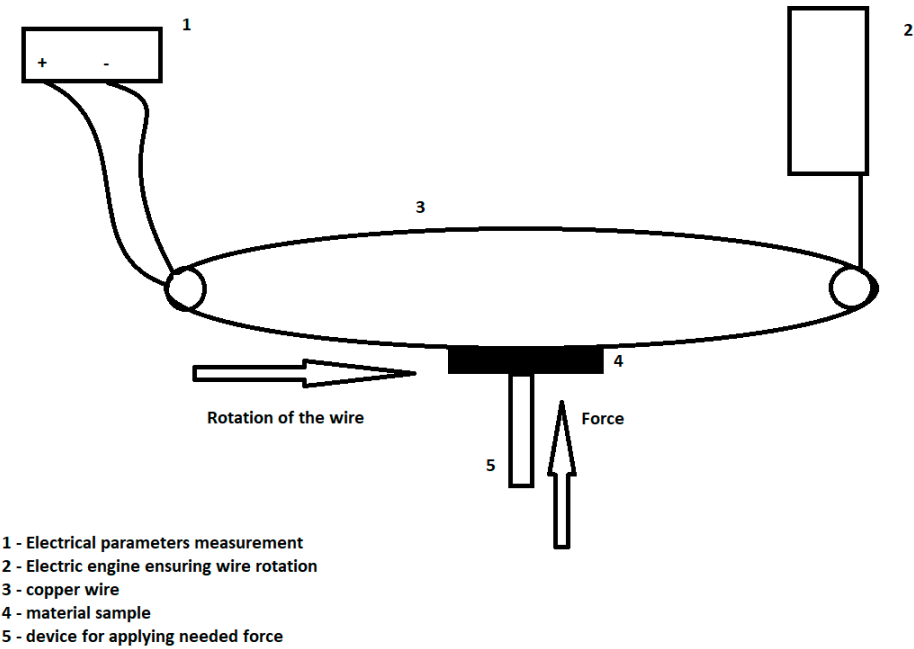
Figure 6. Schematic of functional characterization setup.
