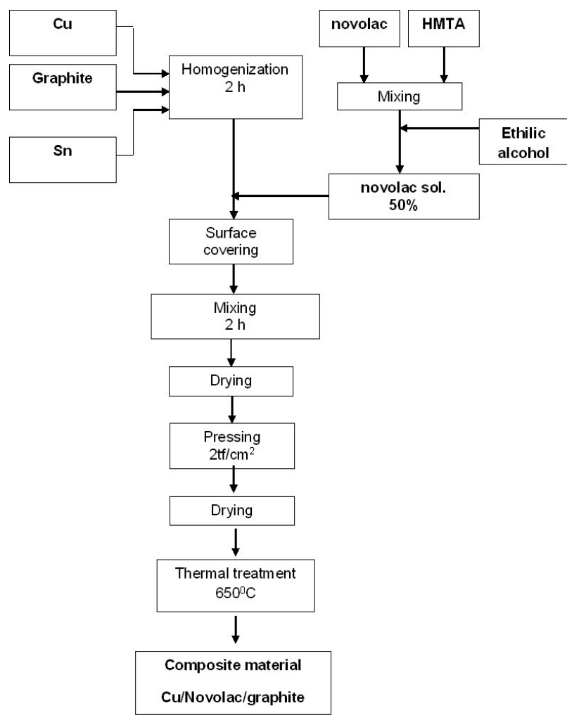
Figure 2. Flow sheet for obtaining Cu/Novolac/Graphite composite material (CGN).
