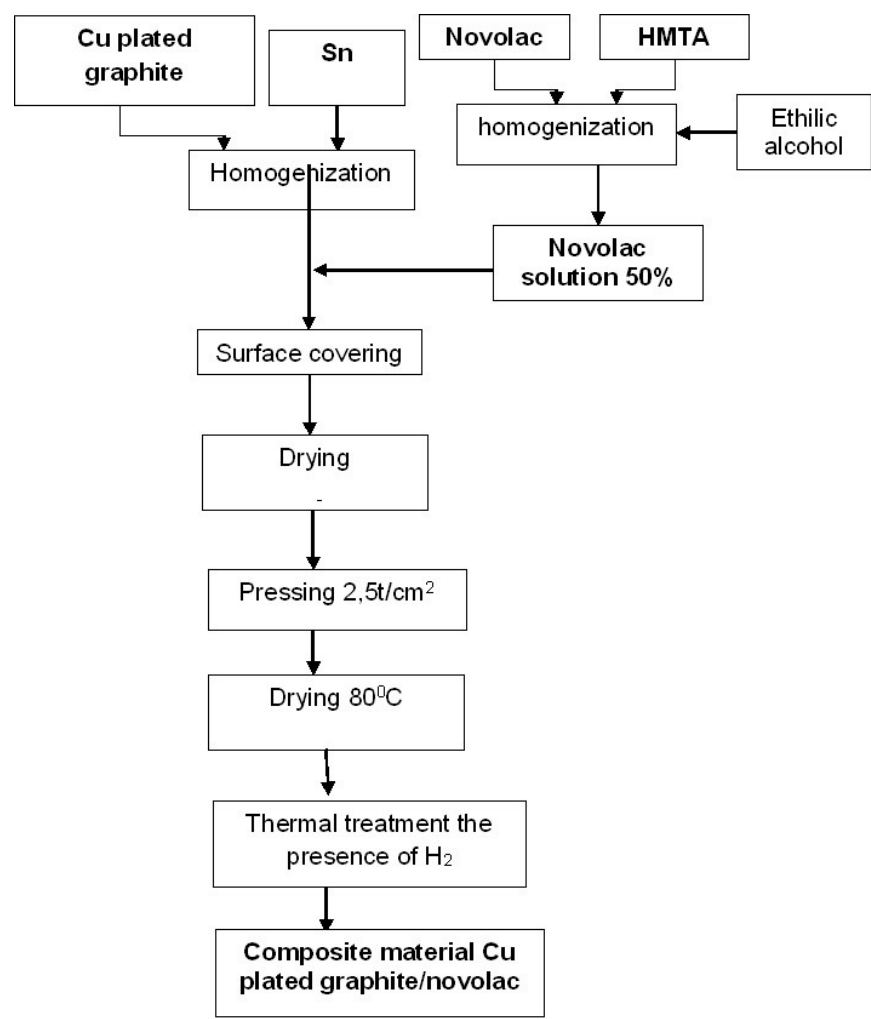
Figure 4. Flow sheet for obtaining Cu plated graphite/Novolac composite material (CGA).
