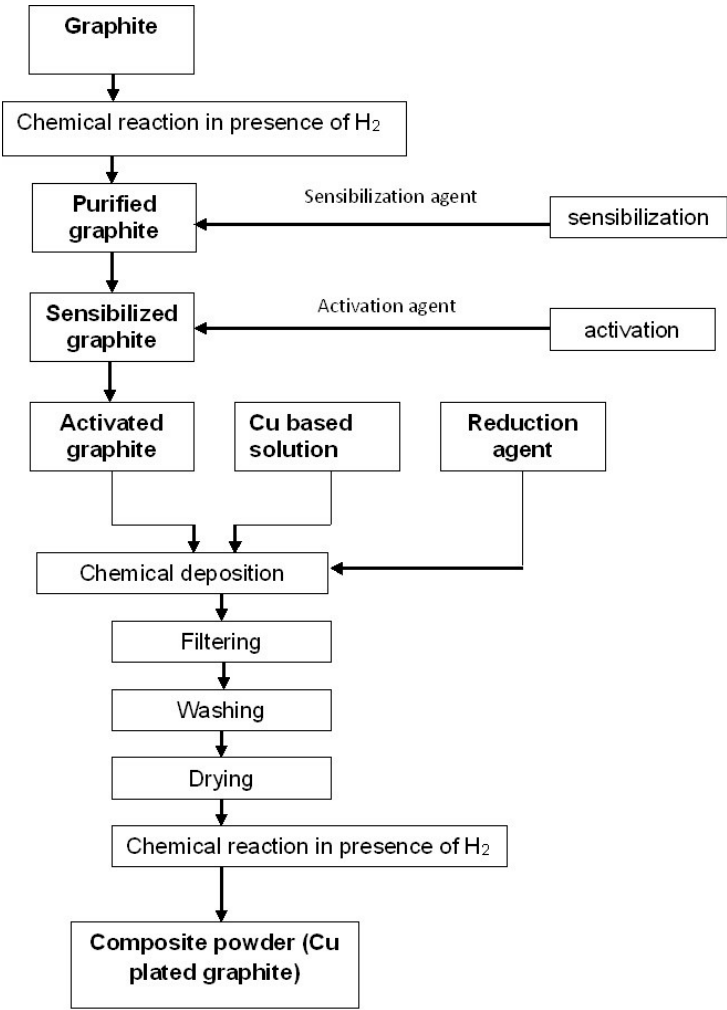
Figure 3. Flow sheet for obtaining Cu plated graphite.
