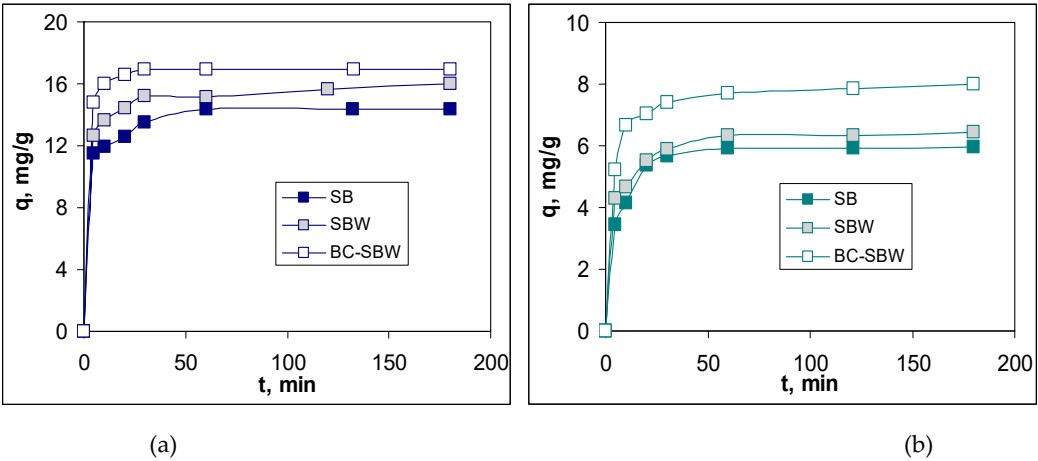
Figure 4. Influence of contact time on the biosorption efficiency of Pb(II) (a) and Cd(II) (b) ions on the three biosorbents (pH = 5.4; biosorbent dose = 4.0 g/L; c_0 = 83.86 mg Pb(II)/L, 46.12 mg Cd(II)/L; temperature = 25 \pm 1 °C).
