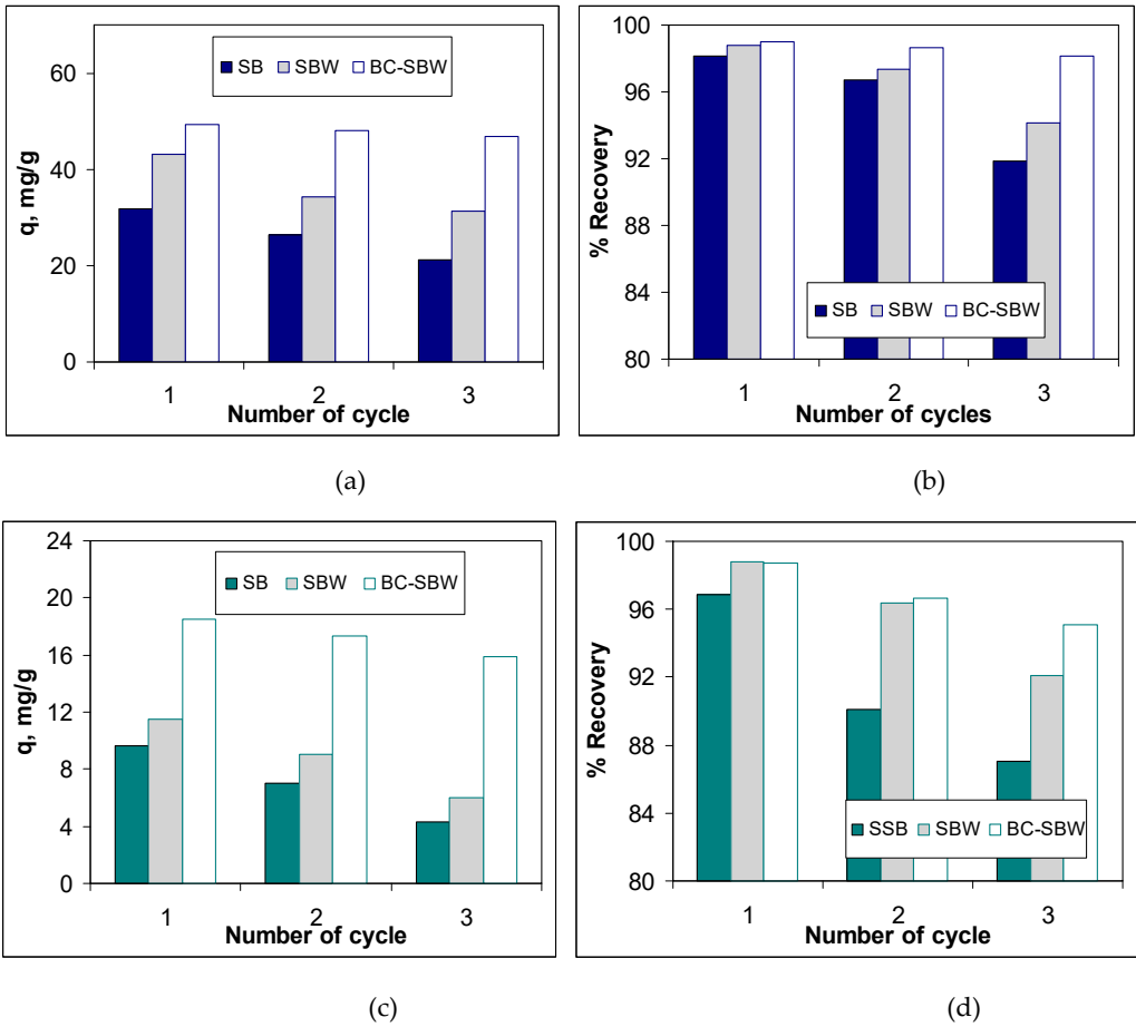
Figure 6. Biosorption (a, c) and desorption (b, d) of Pb(II) ions (a, b) and Cd(II) ions (c, d) on studied biosorbents.
