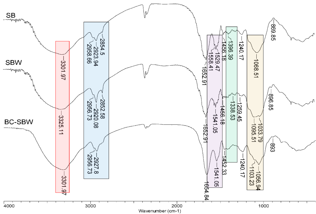
Figure 1. FTIR spectra of SB, SBW and BC-SBW biosorbents.
