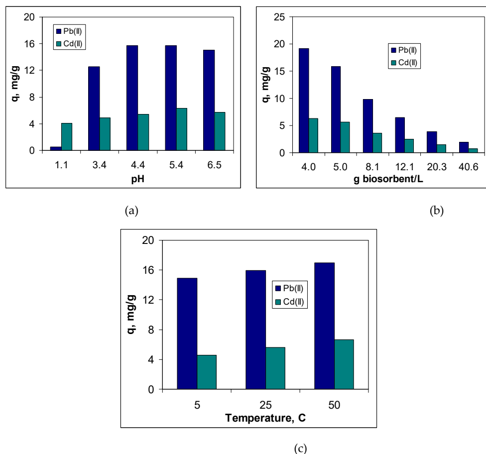
Figure 3. Effect of pH (a), biosorbent dose (b) and temperature (c) on the biosorption efficiency of Pb(II) and Cd(II) ions on SB ( c_0 = 83.86 mg Pb(II)/L, 46.12 mg Cd(II)/L; contact time = 24 h).
