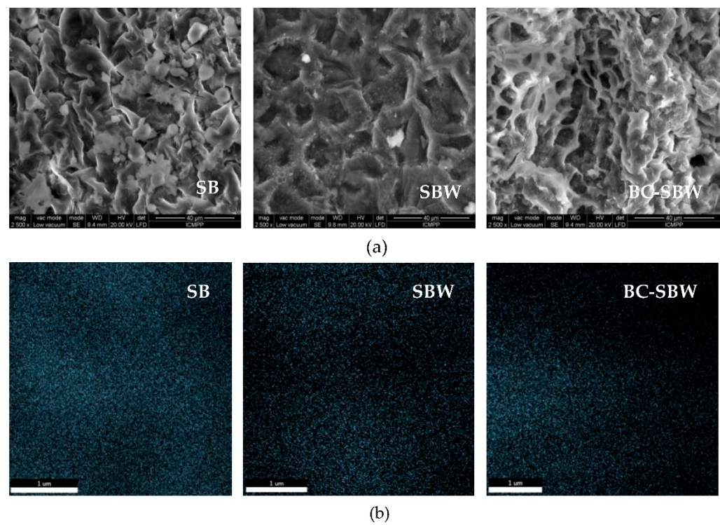
Figure 2. SEM images (a) and oxygen mapping images (b) for SB, SBW and BC-SBW.
