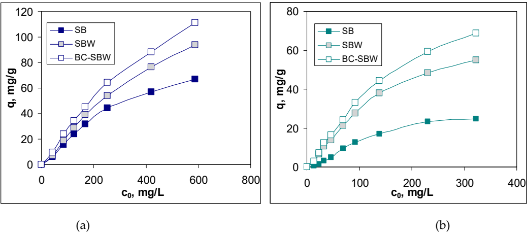
Figure 5. Influence of initial concentration of metal ions on the biosorption efficiency of Pb(II) (a) and Cd(II) (b) ions on the three biosorbents (pH = 5.4; biosorbent dose = 4.0 g/L; contact time = 180 min; temperature = 25 \pm 1 °C).
