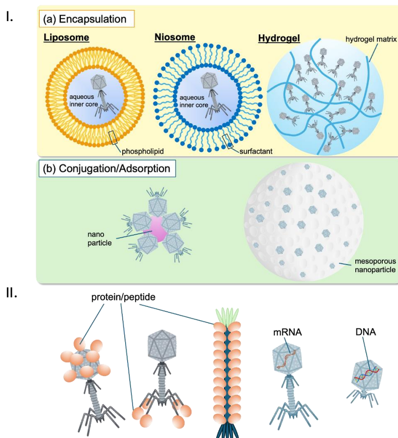
Figure 4. Phage-based drug delivery systems: I. Immobilization of phages: (a) Encapsulation of phage in liposomes (left), niosomes (middle) and in hydrogel beads (right); (b) Conjugation/adsorption of phages onto nano particles (left) and mesoporous nanoparticles (right), respectively. These encapsulation methods protect phages from physicochemical stresses (e.g., pH, shear stress) and/or immunological reactions (e.g., phagocytosis, complement-mediated neutralization). II. Possible drugs delivered by phages as vectors: Proteins (e.g., enzymes, antigens) or peptides can be expressed on the phage capsid, the tips of long tail fibers in Caudovirales, or the major coat proteins in filamentous phages. Additionally, mRNA and/or DNA encoding targeted genes can be loaded into the phage capsid.
