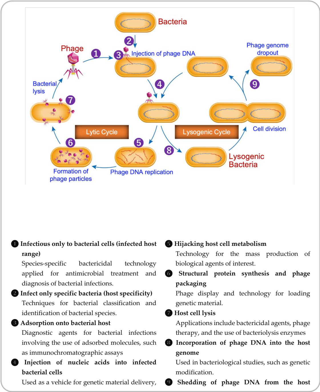
Figure 1. Life cycles of bacteriophages and their applications in medicine. Bacteriophages, or phages, can be divided into two main groups based on their life cycles: lytic phages, which destructively infect and lyse bacterial hosts; and lysogenic phages, which remain dormant within bacteria, replicating their DNA without destroying the host until induced to enter the lytic cycle. These life cycles of phages have been adapted for various uses in medicine, industry, and research.
