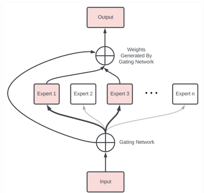
Figure 1. Sparse Mixture of Experts Mixtral 8x22B
