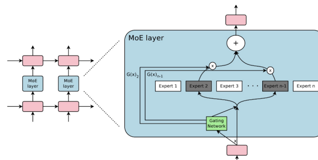
Figure 2. This image illustrates a MoE layer embedded within a recurrent language model [3]. In this case, the sparse gating function selects two experts to perform computations. Their outputs are modulated by the outputs of the gating network
