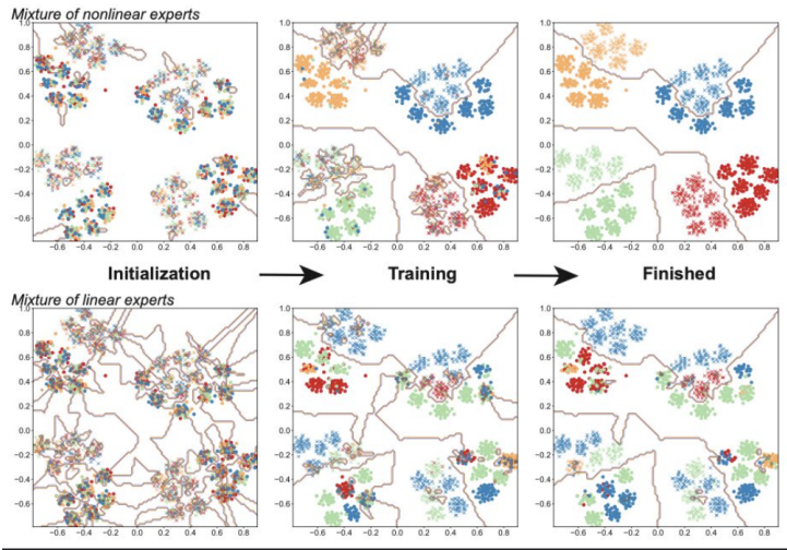
Figure 4. Recent research has started to give us some insights. Here’s a neat visualization from the paper “Towards Understanding the Mixture-of-Experts Layer in Deep Learning” by [74], which shows how a 4-expert MoE model learns to solve a binary classification problem on a toy dataset that’s segmented into 4 clusters.
