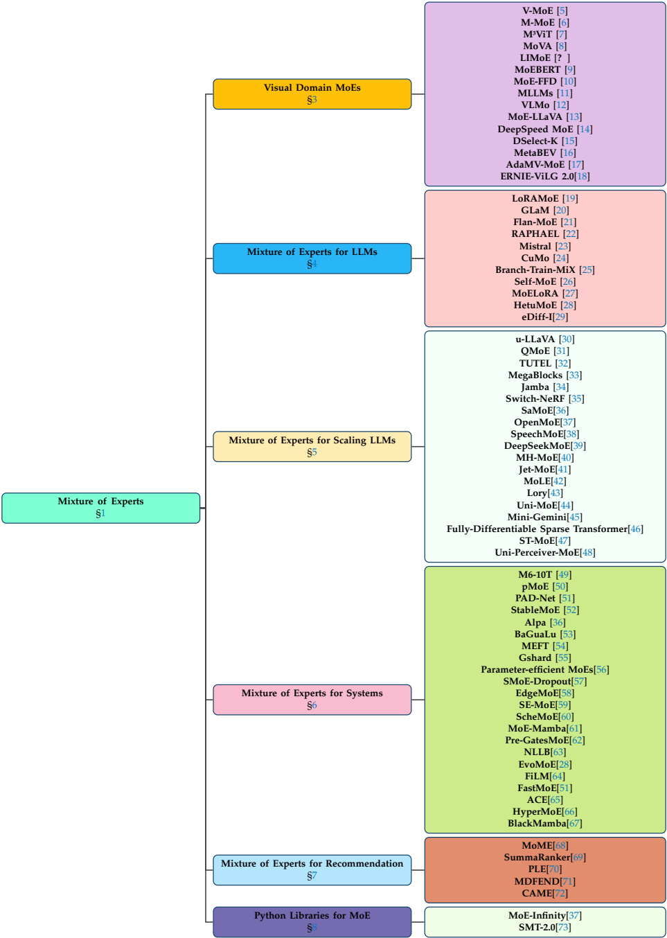
Figure 3. Taxonomy of Mixture of Experts, encompassing Mixture of Experts for Vision,Mixture of Experts for LLMs, Mixture of experts on scaling the LLMs. Mixture of experts in recommendation system and various MoE Python Libraries.
