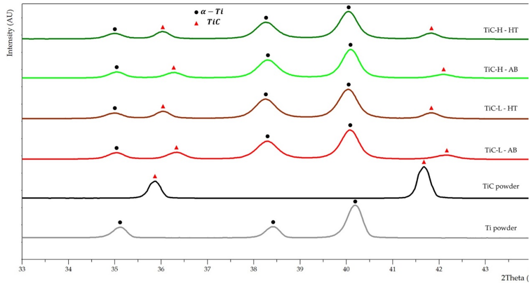
Figure 4. XRD patterns of TiC-L and TiC-H before and after heat treatment as well as reference Ti and TiC powders with 2- \theta angles between 33° and 44°. HT refers to heat-treated samples and AB to as-built ones.
