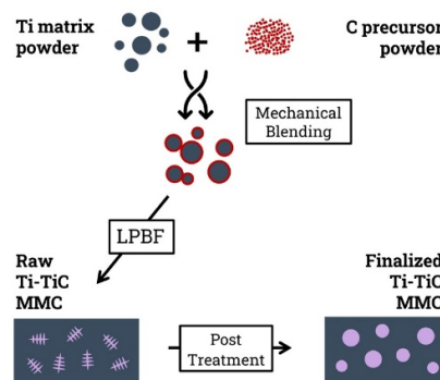
Figure 1. MMC In-situ manufacturing process.
