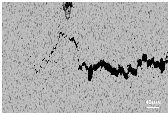
Figure 7. Sub-fracture surface cross-section in TiC-L sample after tensile failure. The cross-section was extracted close to the edge of the fracture surface.
