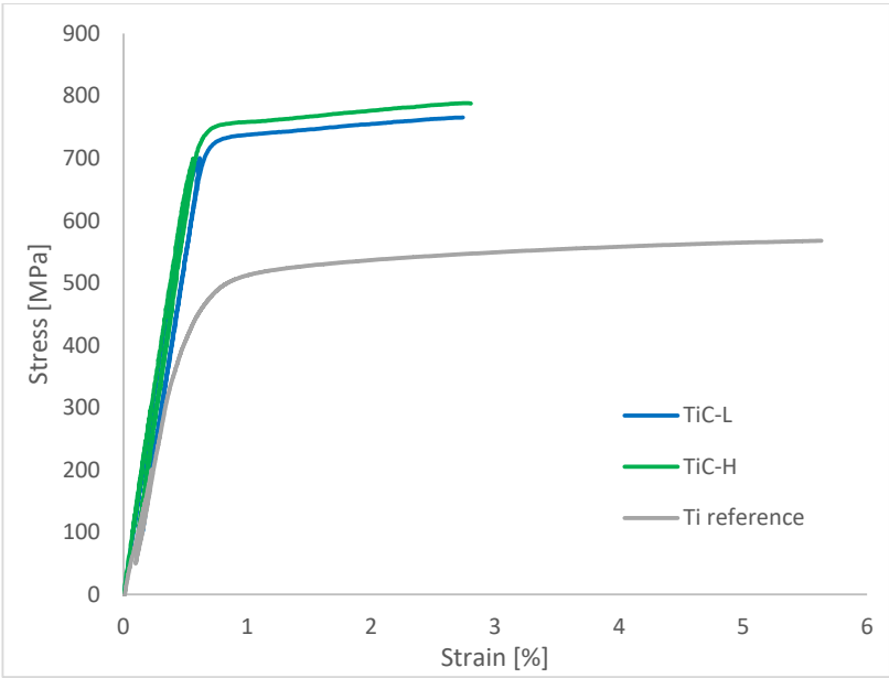
Figure 6. Typical stress-strain curves of TiC-L and TiC-H MMCs as well as Ti reference.
