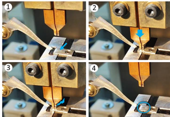
Figure 3. Step by step pictures of the resistance welding process. 1: Placement of sheet metal sample and NiTi wire under weld head 2: Weld head moved down applying pressure on SMA wire with both electrodes; 3: welding current is run through workpieces via copper electrodes; 4: Weld head is moved up and NiTi wire is joined to steel substrate.
