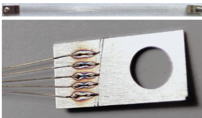
Figure 11. Pictures of a welded SMA wire bundle consisting of five 100 \mu\text{m} wires welded to stainless steel substrates. Upper picture shows a whole bundle with 105 mm wire length. Bottom picture shows a detailed view of the weld spots.
