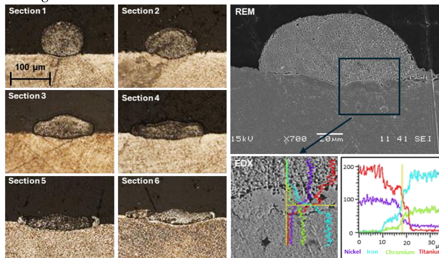
Figure 9. Microscopic analysis of resistance welded NiTi to stainless steel. “Section 1” to “Section 6” show microscopic pictures of samples cut radial to the wire with distances of 100µm in between. On the right a SEM picture of a different sample is displayed with the results of an EDS below.
