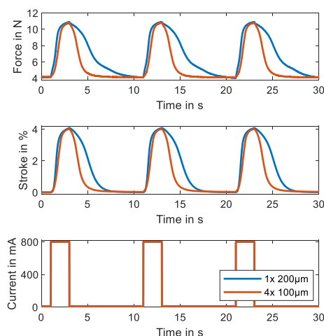
Figure 12. Comparison between bundle of four 100 \mu\text{m} and a single 200 \mu\text{m} diameter wire. Displayed are force, stroke and current over time of three consecutive actuation tests.
