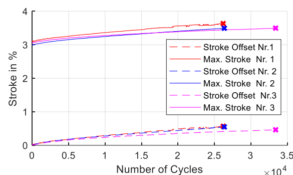
Figure 10. Fatigue test of three samples of 100 µm NiTi wire welded to steel sheet metal. Displayed is maximum and minimum stroke of each cycle until failure.
