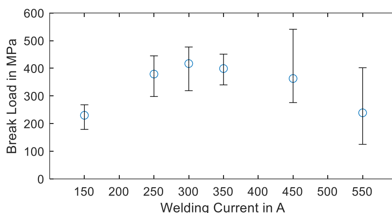
Figure 7. Average values and spread for the joint break loads achieved by peel tests with 100 \mu m NiTi wire resistance step welded to 1.4571 steel sheet metal.
