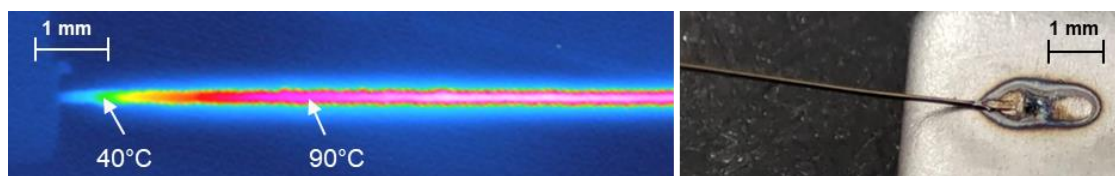
Figure 5. Left: Thermography of a crimped 76 \mu\text{m} NiTi wire, where influence of the heat sink on the temperature distribution in an activated SMA wire is visible. Right: The heat affected zone of a resistance welded 100 \mu\text{m} NiTi to stainless steel is recognized by the tempering colors.
