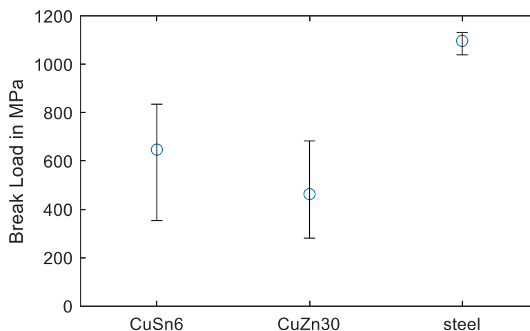
Figure 6. Comparison of the joint break loads of a 100 \mu\text{m} NiTi wire welded to CuSn6, CuZn30 and stainless steel. The results for average value and the spread of the straight pull of tests are displayed.
