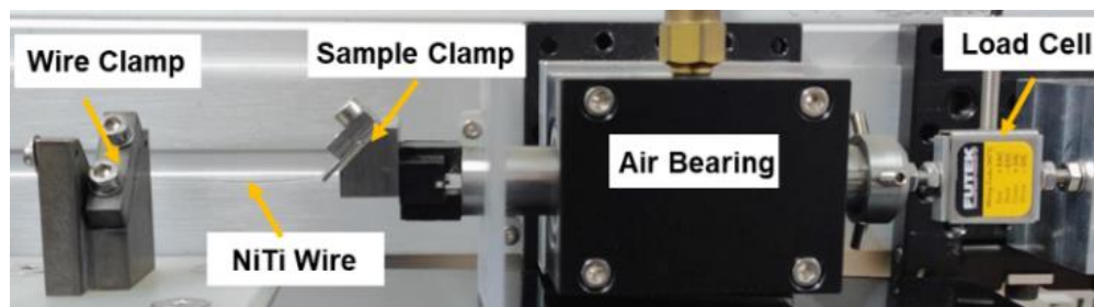
Figure 4. Picture of the test setup for pull-off and peel tests of the welded samples. The sample clamp is replaceable according to the type of experiment.
