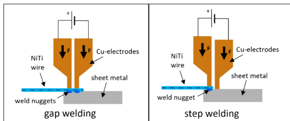
Figure 1. Schematic of resistance gap welding (left) and resistance step welding (right) of NiTi wires to a sheet metal. Displayed are the two copper-based electrodes, pressing down on the work pieces.
