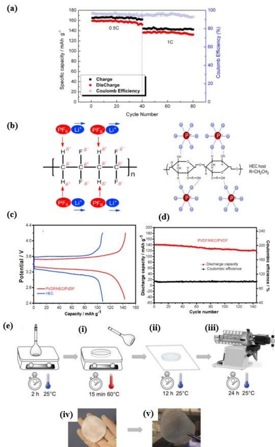
Figure 1. (a) shows the charging discharging discharge cycle functionality of the Li/ILGPE/LiFePO 4 cell at 0.5 C and 1 C rates at 20 °C, reproduced with permission from ref. [29], Elsevier. (b) illustrates interactions occurring in the GPEs: (i) between PVDF and LiPF 6 , and (ii) between LiPF 6 and the hydroxyl groups in the HEC host. LiFePO 4 positive electrode performance with HEC and the composite membrane made of PVDF/HEC/PVDF using 1 mol L -1 LiPF 6 electrolyte, Li metal counter electrode: (c) charge-discharge at 0.2 C, (d) cycling behavior at 0.2 C; reproduced with permission from ref. [30], Elsevier. (e) outlines of GPE membrane preparation: (i) dissolve PVdF in EC: DMC (20:80), stirring 2 hours, (ii) heat, pour into Perti-disk, (iii) age overnight, (iv) vacuum dry 3 hours, (v) display dry PVdF precursor, reproduced with permission from ref. [31], Elsevier.
