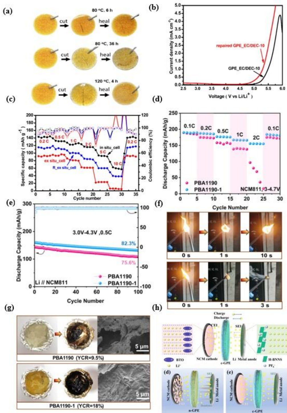
Figure 11. (a) Showing self-healing of GPE_EC/DEC-10 under different thermal treatments. (b) Comparison of linear sweep voltammety curves before and after a cut-self-healing process in GPE_EC/DEC-10. (c) cycling at various C rates, adopted from ref. [67]. (d) The rate performance with PBA1190 and PBA1190-1. (e) The cycle performance with PBA1190 and PBA1190-1 in the voltage range at 0.5 C for 100 cycles (f) Combustion tests of PBA1190 (i) and PBA1190-1 (ii) electrolytes in air. (g) Images of residual char following the thermal oxidation degradation of PBA1190 (i) and PBA1190-1 (ii) electrolytes at 500 °C for 0.5 hours, reproduced with permission from ref. [92], Elsevier. (h) displays HRTEM analyses of NCM-523 cathodes from Li/NCM-523 cells with n-GPE and c-GPE-2
