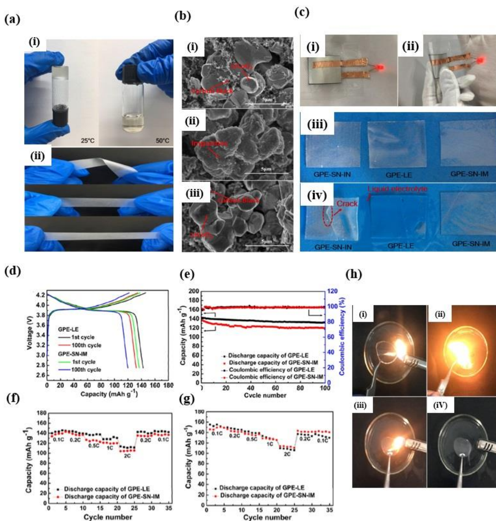
Figure 8. (a) (i) Shows SN electrolytes at 25 °C and 50 °C, highlighting the change from a paste-like to a liquid state. (ii) displays the flexible and stretchable characteristics of the GPE-SN-IM film. (b) shows SEM images of the fresh LiCoO 2 cathode and the cathodes from cells utilizing GPE-LE and GPE-SN-IM after 100 charge-discharge cycles at 55 °C, showing differences (c) (i) Battery lighting up an LED with LiCoO 2 /GPE-SN-IM/Li 4 Ti 5 O 12 . (ii) GPE-SN-IM battery still powers LED after 100 folds. (iii) Discharge capacities with different GPEs before folding. (iv) Discharge capacities after 100 folds, GPE-LE shows electrolyte leakage. (d-g). Charge-discharge characteristics of LiCoO 2 /Li cells built with GPE-LE and GPE-SN-IM at a different condition. (h) Flame ignition tests for (i) GPE-LE and (iii) GPE-SN-IM. After contacting the flame, (ii) GPE-LE quickly burns but (iv) GPE-SN-IM does not burn; Reprinted with permission from [49]. Copyright © 2018, American Chemical Society.
