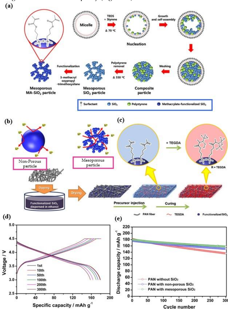
Figure 5. (a) Synthesis of mesoporous MA-SiO 2 particles (b) Varied lithium-ion transport characteristics with non-porous and mesoporous MA-SiO 2 particles in the composite gel polymer electrolyte. (c) Displays the development of the cross-linked composite gel polymer electrolyte utilizing a fibrous PAN membrane, mesoporous MA-SiO 2 nanoparticles, and a gel electrolyte precursor featuring TEGDA. (d) Charge and discharge profiles of a lithium-ion polymer cell utilizing a cross-linked composite gel polymer electrolyte with mesoporous MA-SiO 2 nanoparticles, and (e) Discharge capacities of lithium-ion polymer cells using various electrolytes at 25 °C, adopted from ref. 44.
