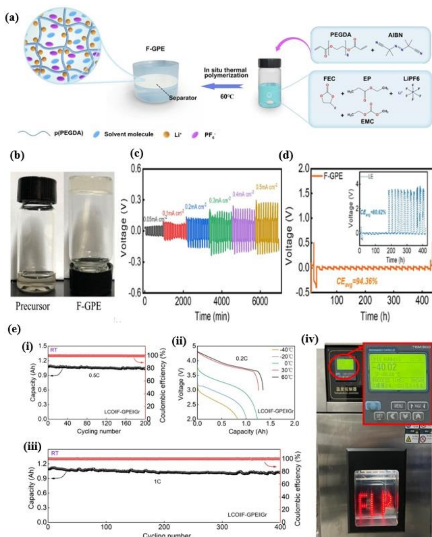
Figure 6. (a) The method for preparing F-GPE. (b) Visual representations of F-GPE. (c) Voltage-time profile for the plating/stripping process of a symmetric Li||F-GPE||Li cell at different current densities. (d) The CE avg of Li||FGPE||Cu cell at 0.5 \text{ mA cm}^{-2} . (e): (i) Cycling performance of LCO at room temperature. (ii) Discharge curves of LCO at different temperatures. (iii) Long-term cycling performance of LCO after 400 cycles at ambient temperature. (iv) Photo of LCO pouch battery lighting 70 LEDs at -40^\circ\text{C} ; reproduced with permission from ref. [45], Elsevier.
