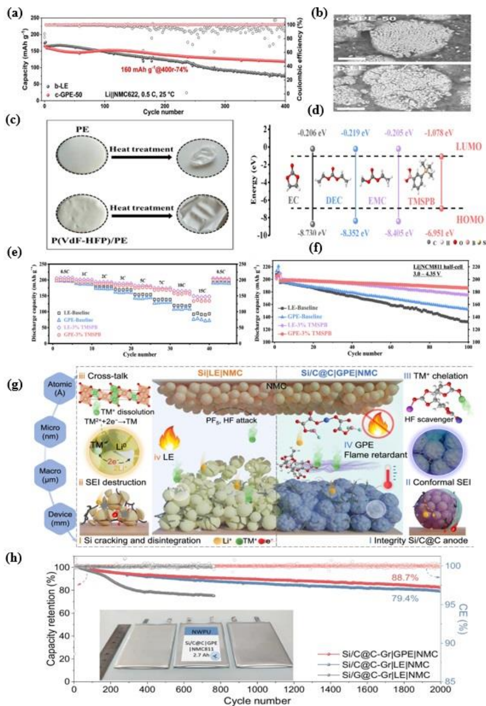
Figure 12. (a) Cycling performances of the Li||NMC622 batteries with b-LE and c-GPE-50 at 0.5 C. (b) SEM images, reproduced with permission from ref. [95], Elsevier. (c) Optical images of PE and P(VdF-HFP)/PE membranes before and after 30 min heat treatment at 135 °C. (d) illustrates the Optimized structures and LUMO/HOMO energies of carbonate solvents (EC, DEC, EMC) in liquid electrolyte and TMSPB additive. (e) displays the cycling of Li||NCM811 half-cells with various electrolytes at different charge rates in the voltage range of 3.0–4.35 V. (f) shows the rate capability of Li||NCM811 cells in different electrolytes; Reprinted with permission from [99]. Copyright © 2022, American Chemical Society. (g) Illustrates a Si-based anode||NMC full cell model, showing the fading mechanisms in the Si|LE|NMC prototype, including Si cracking, Li + depletion, SEI rupture, and safety hazards. It also highlights the features of the Si/C@C|GPE|NMC system, emphasizing the Si/C@C anode design with improved interfacial stability, suppressed crosstalk effect, and flame retardancy of the GPE. (h) displays electrochemical performance of the Si/C@C-Gr|GPE|NMC full cell, focusing on the cycling behavior of the cells, adopted from ref. [100] Springer Nature.
