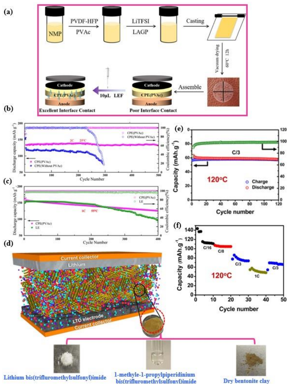
Figure 10. (a) A schematic of the preparation process for CPE(PVAc) and its battery configuration. (b) Comparison of long-term cycling performance between LiFePO 4 |CPE(PVAc)|Li and LiFePO 4 |CPE (without PVAc)|Li at a rate of 2 C and a temperature of 25 °C. (c) Long-term cycling performance comparison of LiFePO 4 |CPE(PVAc)|Li and LiFePO 4 |LE|Li at a rate of 1 C and 55 °C, reproduced with permission from ref. [65], Elsevier. (d) shows the components used to create the clay-RTIL quasi-solid-state electrolyte and the structure of the LIB. (e) illustrates both the cyclic stability and rate capability of Li 4 Ti 5 O 12 half cells at 120°C; Reprinted with permission from [66]. Copyright © 2015, American Chemical Society.
