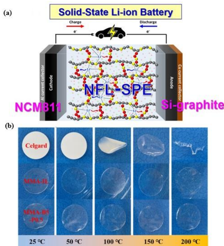
Figure 13. (a) Schematic of a Si-graphite/NFL-SPE/NCM811 solid-state Li-ion full cell (see Figure 14a), reproduced with permission from ref. [101], Elsevier. (b) Images depicting thermal shrinkage for the Celgard separator, MMA-IL, and MMA-B5-P0.5 reproduced with permission from ref. [102], Elsevier.
