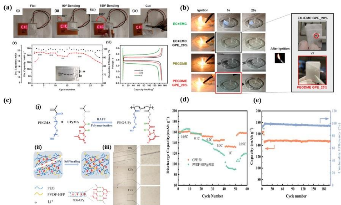
Figure 3. (a) Displays flexibility and safety tests of the Li 0 /GPE 20 %/LFP pouch cell using LED lighting: (i) initial state, (ii) at 90°, (iii) at 180°, and (iv) post-cutting. It also includes (v) battery performance and (vi) charge/discharge characteristics at different C-rates. (b) illustrates the flammability test conducted on EC+EMC and PEGDME solvents alongside their respective gel polymer electrolytes; adopted from ref. [33]. (c) (i) Represents the schematic synthesis process of the brush-like copolymer PEG-UPy. (ii) Illustrates the formation of PP-PU along with its self-healing mechanism at the surface of the cut. (iii) Presents optical images illustrating the self-healing process of PP-20PU samples under normal conditions. (d) Compares the discharge-specific capacity of Li/GPE-20/LFP and Li/PVDF-HFP@PEO/LFP configurations cells across different rates. (e) Demonstrates the cycling efficiency and Coulombic efficiency of Li/GPE-20/LFP cells when tested at 1 C. Reprinted with permission from [34]. Copyright © 2022, American Chemical Society.
