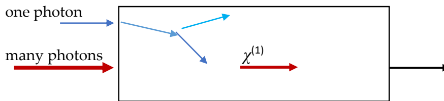
Figure 1. Schematic of one photon being randomly scattered inside a dielectric medium, while a group of identical photons propagates in a straight-line.
